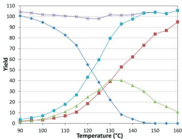
Fig. 3 Silicon reactor, \tau = 3 min, P_{CO} = 8.3 bar, using p -bromobenzonitrile. Aryl bromide starting material (◆), amide product (■), \alpha -keto amide product (▲), total product (●), and mass balance (×).
