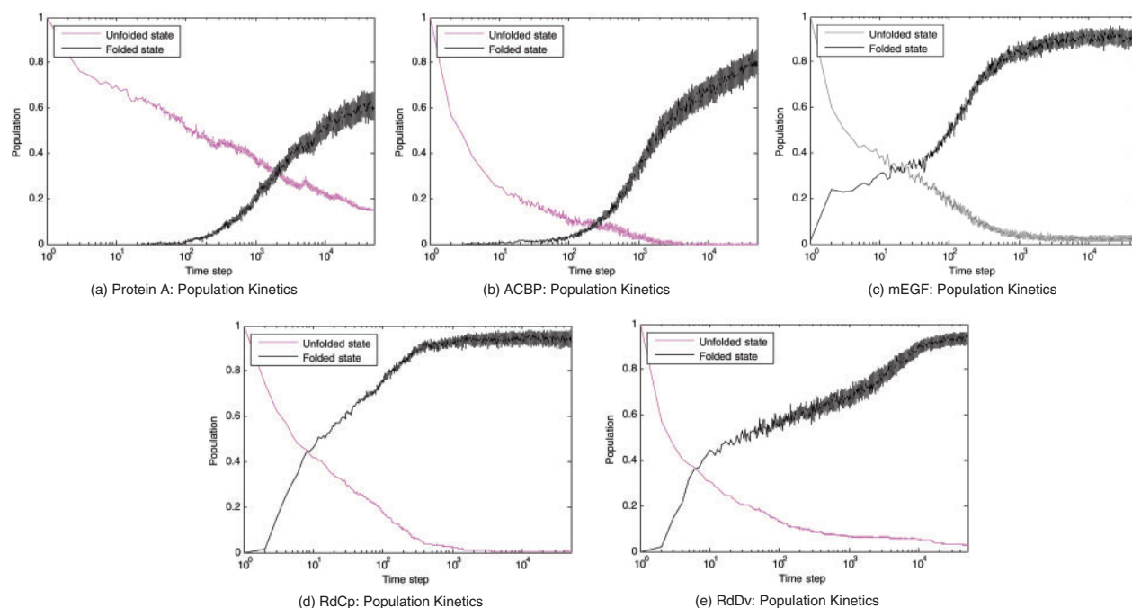
Fig. 2. Population kinetics from MMC simulations for proteins in Table 1 of varying structure: (a, b) \alpha , (c) \beta , (d, e) mixed.
