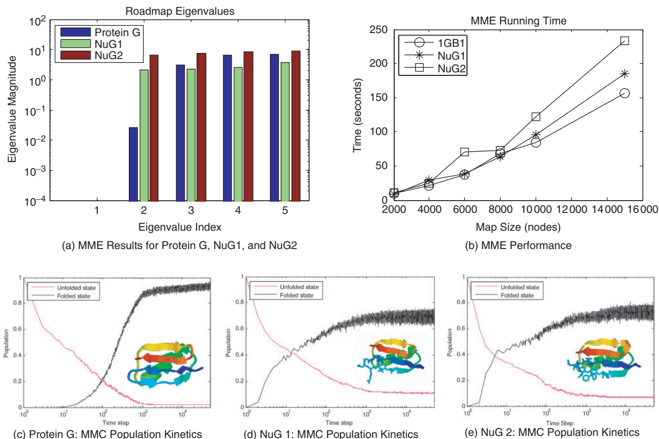
Fig. 1. (a) Eigenvalue comparison between protein G and mutants NuG1 and NuG2 computed by MME. NuG1 and NuG2 are experimentally known to fold 100 times faster than protein G (Nauli et al. , 2001). (b) Running time of MME for protein G and mutants NuG1 and NuG2 as a function of roadmap size. MME scales linearly with the landscape model/map size. (c–e) Population kinetics from MMC for protein G and mutants NuG1 and NuG2. As with MME, the MMC results also indicate that the mutants fold faster than wild-type. Ribbon diagrams show mutated hairpin in wireframe.
