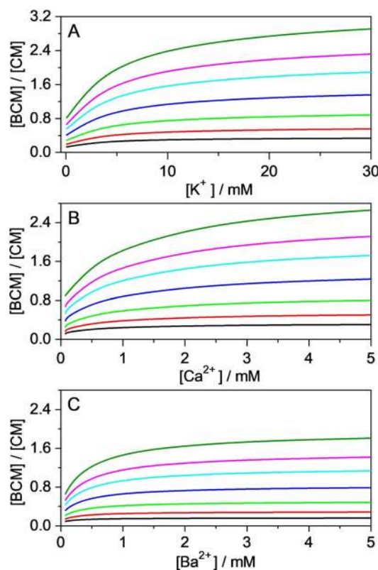
Figure 6. Variation of B^+-CB7-M^{n+}/CB7-M^{n+} molar ratios in equilibrium as a function of A) K^+ , B) Ca^{2+} and C) Ba^{2+} concentrations in equimolar solutions of B^+ and CB7. [B^+] = [CB7] = 15, 10, 7, 4, 2, 1, and 0.5 \mu M (from top to bottom).
