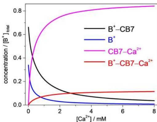
Figure 5. Composition of solutions at various Ca^{2+} concentrations and [B^+]_{total} = [CB7]_{total} = 0.25 \mu M .
