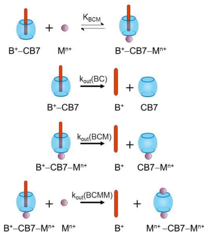
Scheme 3. Mechanism of B + release from the CB7 cavity.
