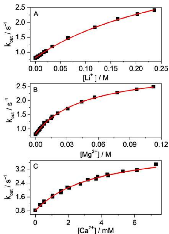
Figure 2. Effect of A) LiCl, B) MgSO 4 and C) CaCl 2 concentrations on the apparent rate constant of B + release from CB7. Lines represent the fitted function.
