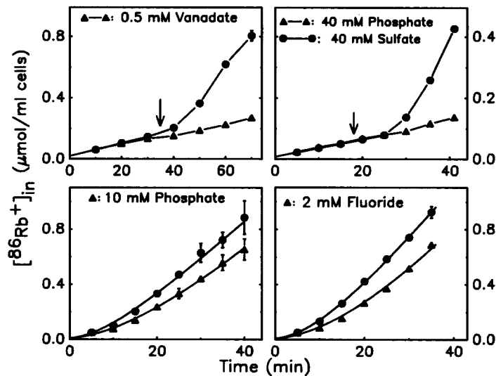
FIGURE 9. Inhibition of swelling-stimulated ^{86}\text{Rb}^+ influx by orthovanadate, phosphate, and fluoride. Upper left : Cells were incubated 15 min in 150 mM NaCl, 10 mM HEPES, 10^{-4} M ouabain, with or without 0.5 mM vanadate before addition of ^{86}\text{RbCl} with 5 mM KCl at t = 0 . At the arrow, the osmolality was lowered to 210 mosmol. Triangles represent the suspensions with vanadate. The intracellular vanadate concentration is unknown but is less than the extracellular concentration, because the Donnan ratio is less than unity and because of reduction of vanadate (Macara et al., 1980). Data shown are mean and range of duplicate determinations. Upper right : Same as upper left, except that 55 mM of the NaCl was replaced with either 40 mM \text{Na}_2\text{SO}_4 or 40 mM \text{Na}_2\text{HPO}_4/\text{NaH}_2\text{PO}_4 . The comparison of sulfate with phosphate was performed to ensure that the phosphate inhibition is not caused by removal of some of the chloride. Single experiment representative of three. Lower left : Cells were swollen simultaneously with ^{86}\text{Rb}^+ addition. The triangles represent suspensions in which 10 mM NaCl was replaced by 8 mM \text{Na}_2\text{HPO}_4/2 mM \text{NaH}_2\text{PO}_4 40 min before the beginning of the influx measurement. Lower right : Same as lower left, except 2 mM NaF replaced 2 mM NaCl 1 min before the influx began. Similar results were obtained in three other experiments.
