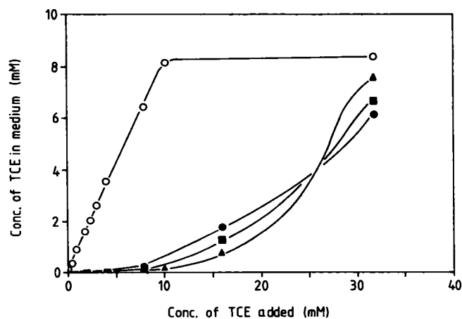
FIG. 2. Effect of addition of different types of PAC (5 g liter -1 ) on the adsorption of TCE under degradation conditions, as described in Materials and Methods. Symbols: ■, PAC type SA4; ●, PAC type D10; ▲, PAC from Baker; ○, no PAC added.
