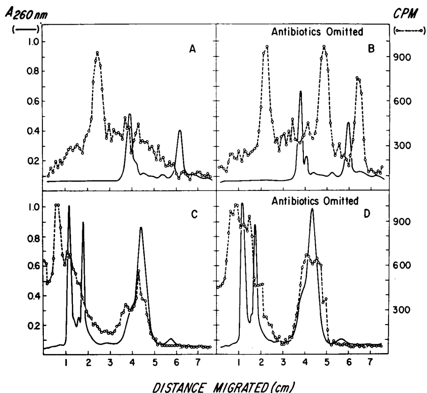
FIGURE 6 Effect of resident bacteria on labeling patterns. Labeling was for 2 hr in vitro with uridine- 3 H. Slower-migrating species (electrophoresis for 5 hr) in bladders treated with penicillin and streptomycin (A) are compared with species from bladders not so treated (B). Faster-migrating species (electrophoresis for 1.5 hr) are also shown with (C) and without (D) penicillin and streptomycin.
