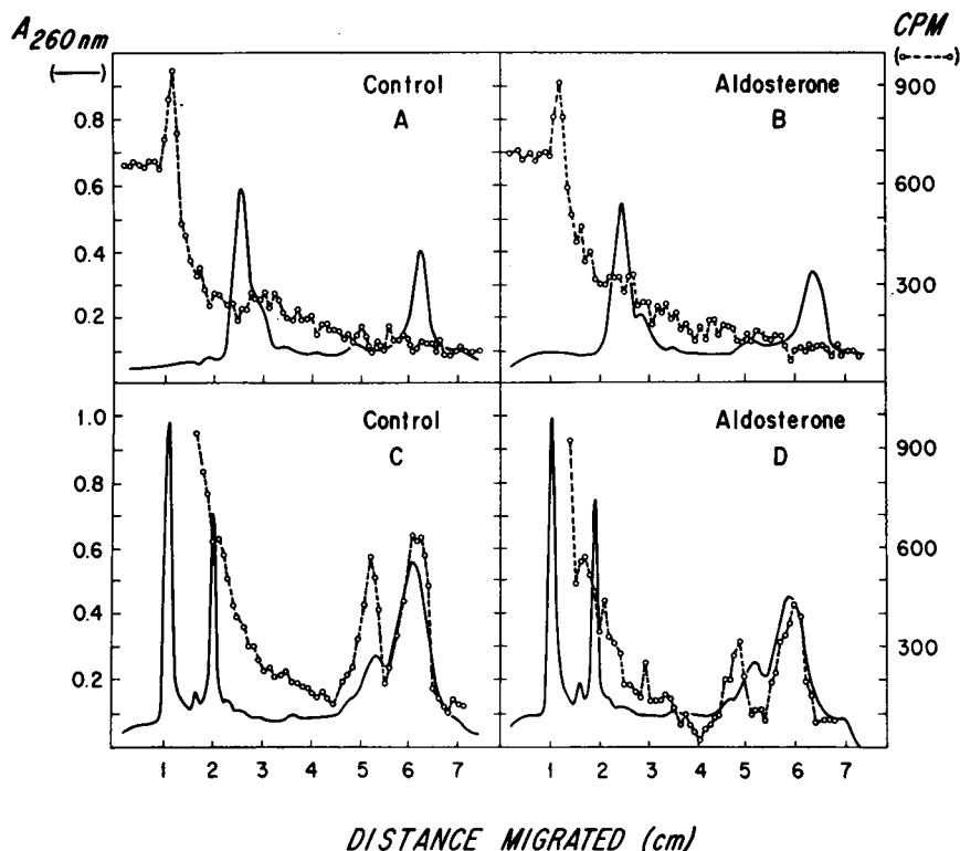
FIGURE 5 Labeling after treatment with aldosterone ( 5 \times 10^{-7} mole/liter). Continuous labeling was with uridine- ^3\text{H} in vitro for 1 hr. Slower-migrating species (electrophoresis for 5 hr) are shown without (A) and with (B) aldosterone added. Faster-migrating species (electrophoresis for 1.5 hr) are shown without (C) and with (D) aldosterone.
