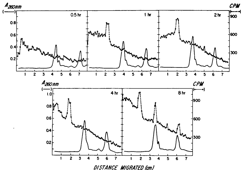
FIGURE 1 Kinetics of labeling in slower-migrating RNA. Hemiblasters were labeled continuously with uridine- ^3H in vitro and processed as described in the text. RNA was run on 7-cm 2.65% polyacrylamide gels (5 ma/gel, 10 v/cm) for 5 hr, scanned at 260 nm, and analyzed for radioactivity.
