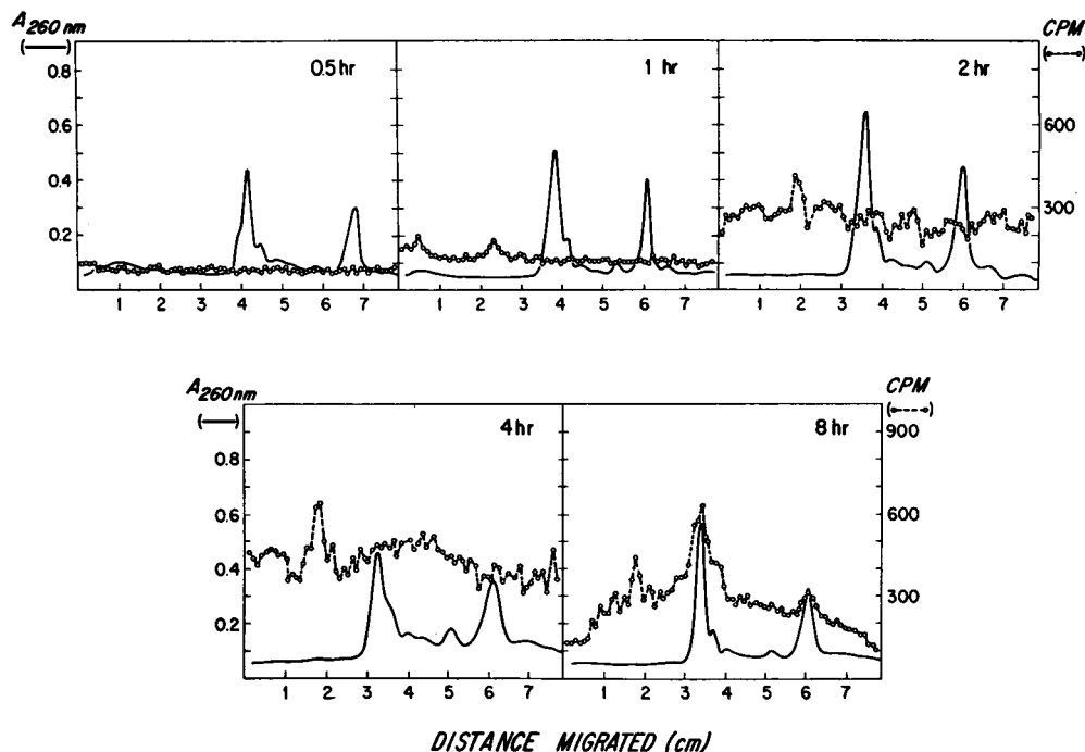
FIGURE 2 Kinetics of labeling of methylated RNA. Details were as in Fig. 1 except that the precursor was methionine-(methyl)- ^3\text{H} .
