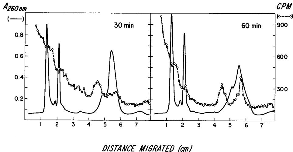
FIGURE 4 Labeling in rapidly migrating RNA. The precursor was uridine- 3 H in vitro and electrophoresis was for 1.5 hr.
