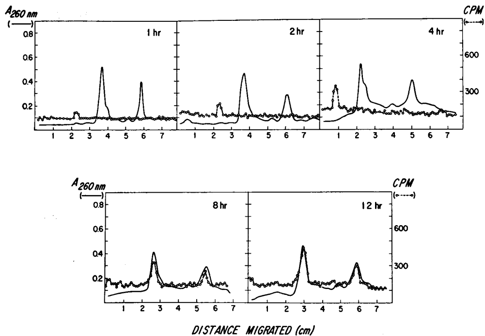
FIGURE 3 Kinetics of labeling in vivo. The technique was identical to that in Fig. 1 except that the uridine- ^3\text{H} was given parenterally.
