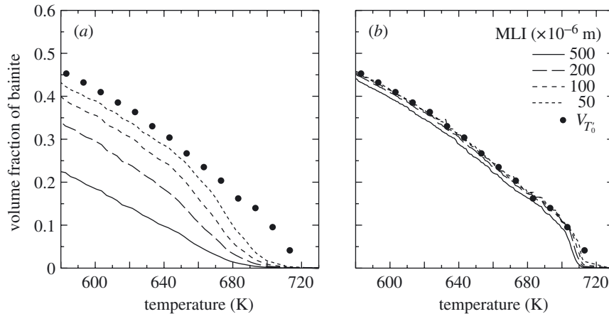
Figure 10. Effect of the austenite grain size on the volume fraction of bainite in continuous cooling transformation. Cooling rates are (a) 6.67 \times 10^{-2} \text{ K s}^{-1} and (b) 5.83 \times 10^{-3} \text{ K s}^{-1} .
