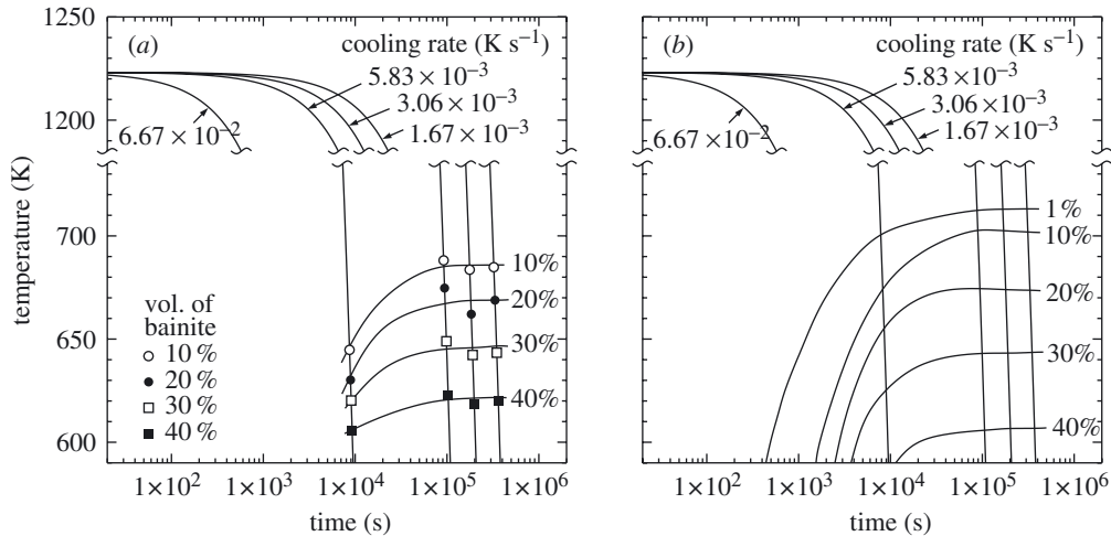
Figure 9. Continuous cooling transformation curves of steel 3: (a) evaluated by interpolating the experimental data by Khan & Bhadeshia (1990); (b) calculated using this model.
