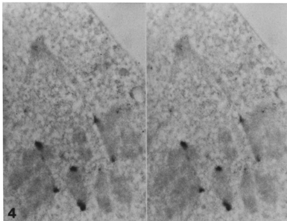
FIGURE 4 High-voltage stereo electron micrographs of a thick-sectioned metaphase cell. The kinetochores are densely and specifically stained. \times 7,000 .
