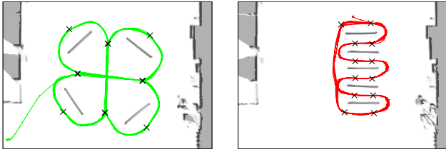
Fig. 6. Trajectory of a Pioneer P3-DX robot overlaid on a grid map for the obstacle courses “clover” (left) and “zigzag” (right). The crosses mark intermediate goal locations. The robot drove 10 rounds in the clover course, and 5 rounds in the zigzag course. The frames cover an area of 14m x 10m.
