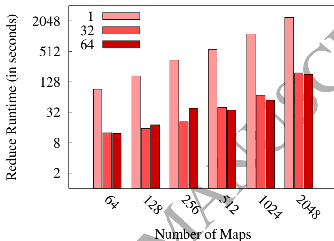
Figure 10: Reduce Runtime vs. number of maps and reducers — SUSY
