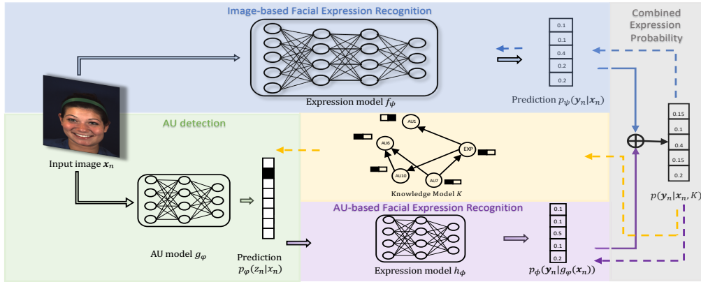
Figure 1: Overview of the proposed framework. Dotted lines represent back-propagation steps for each module.
