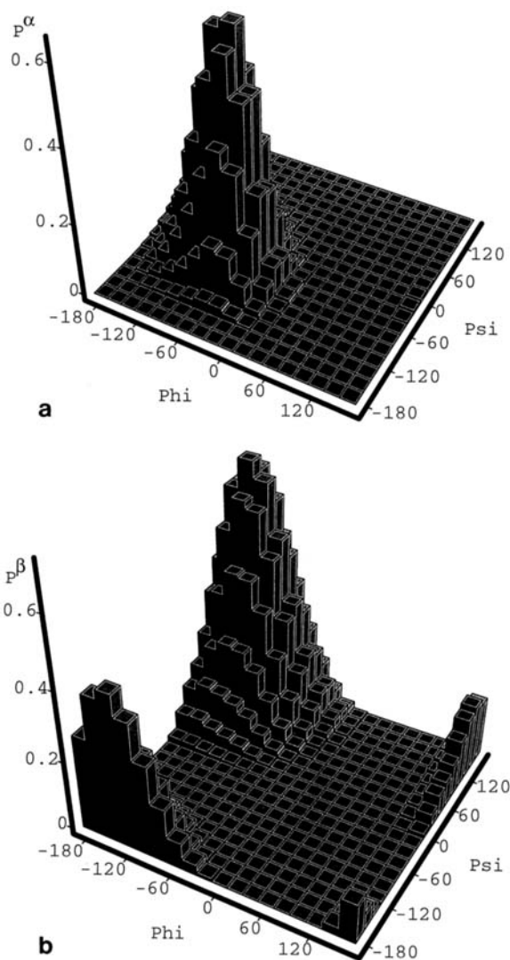
Fig. 2. Probabilities P^{\alpha} (a) and P^{\beta} (b) for residues in \alpha -helical and \beta -sheet secondary structural state, respectively, to have different torsional angles \varphi and \psi . The histograms are given for 20^{\circ} -by- 20^{\circ} zones.
