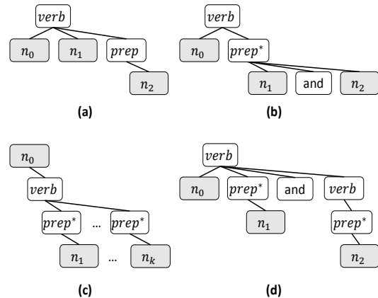
Figure 5: Four syntax-based patterns for question decomposition
