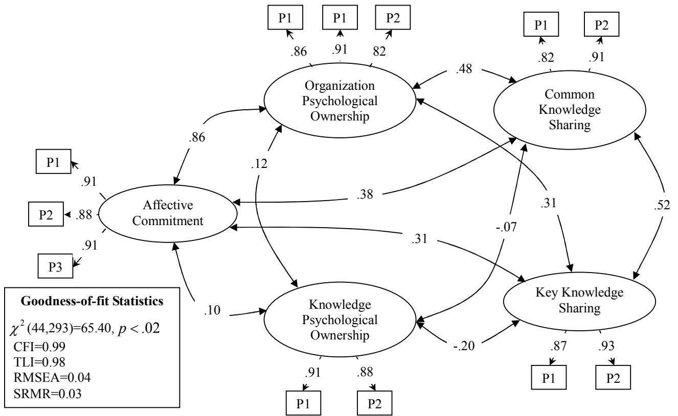
Figure 1. Hypothesized measurement model
