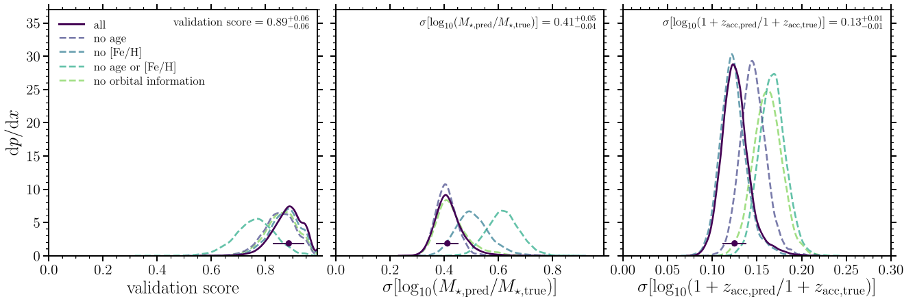
Figure 1. Validation of the neural network. Left: PDF of validation scores across all 10 000 Monte Carlo realizations of the neural network, for models including different subsets of the feature variables as indicated by the legend. The data point with error bar and the annotation in the top right indicate the median and 16–84th percentiles for the experiment including all feature variables. Middle: PDF of the logarithmic scatter of the predicted stellar masses of the satellite progenitors around their true stellar masses. Lines and annotation as in the left-hand panel. Right: PDF of the logarithmic scatter of the predicted accretion redshifts of the satellite progenitors around their true accretion redshifts. Lines and annotation as in the left-hand panel. This figure shows that the neural network performs well, predicting stellar masses ( M_* ) within a factor of 2.5 and accretion redshifts ( 1 + z_{\text{acc}} ) within a factor of 1.35.
