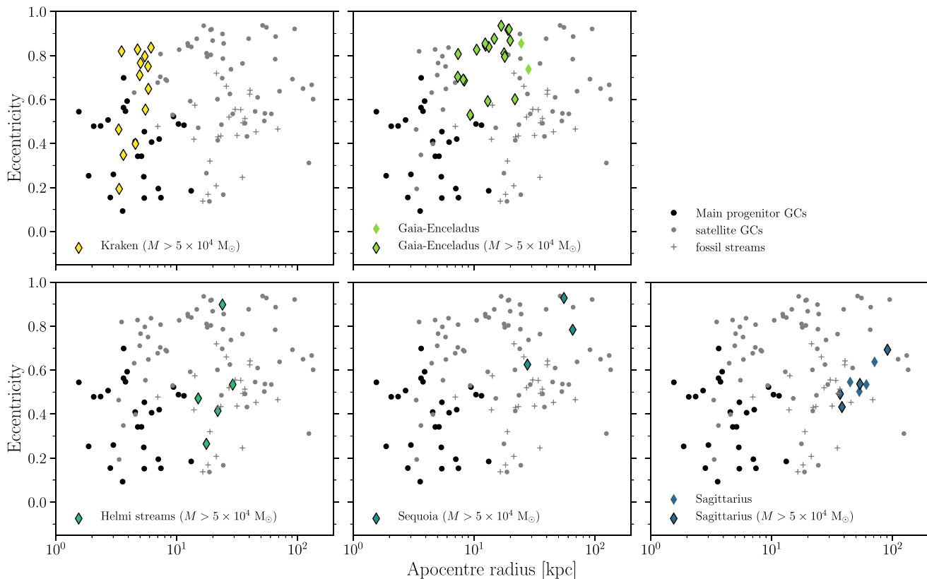
Figure 2. Orbital properties of the Galactic GC population, expressed in terms of their apocentre radii and eccentricities. In all the panels, we distinguish GCs that formed in the Main progenitor and those that formed in satellites (largely following Massari et al. 2019, with changes as discussed in the text), as well as fossil streams that are likely relics of GCs (taken from Bonaca & Kruijssen, 2020), which we do not associate to any specific accretion event here. In each of the panels, the unambiguous members of each satellite progenitor are highlighted, demonstrating that GCs associated with different satellite progenitors have different orbital properties.
