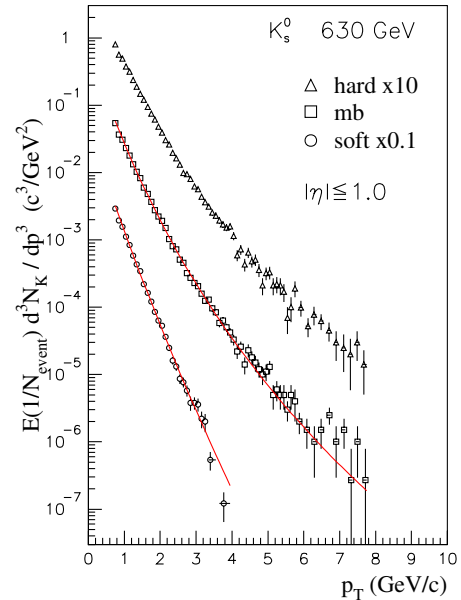
FIG. 8 (color online). K_S^0 inclusive invariant p_T distributions at 630 GeV MB, soft , and hard data are shown, normalized to the number of events in each sample. E is the particle energy and N_{\text{event}} is the total number of events which contribute to the distribution. To separate the curves, hard data points are multiplied by 10 and soft data points by 0.1. The solid lines represent the best fits to Eq. (2) of the text.
