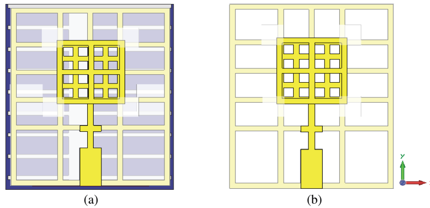
Figure 5. Proposed suspended meshed patch antenna (a) with solar cell (b) without solar cell and cover glass (with only meshed ground plane).
