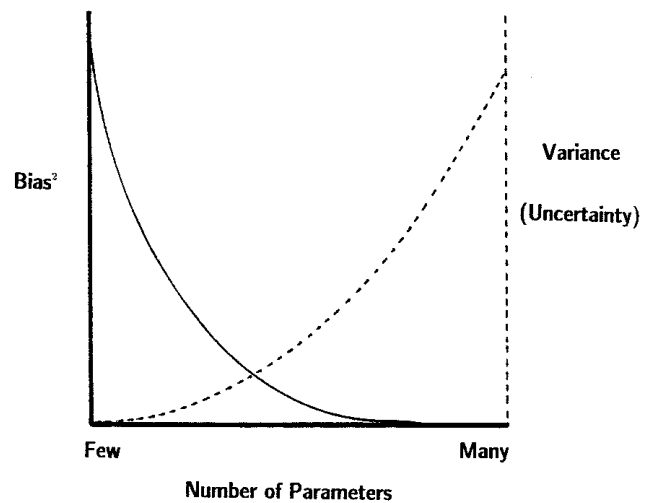
Fig. 1. The principle of parsimony: the conceptual trade-off between squared bias (solid line) and variance (i.e. uncertainty) versus the number of estimable parameters in the model. The best model has dimension ( K_0 ) near the intersection of the two lines, while full reality lies far to the right of trade-off region.
