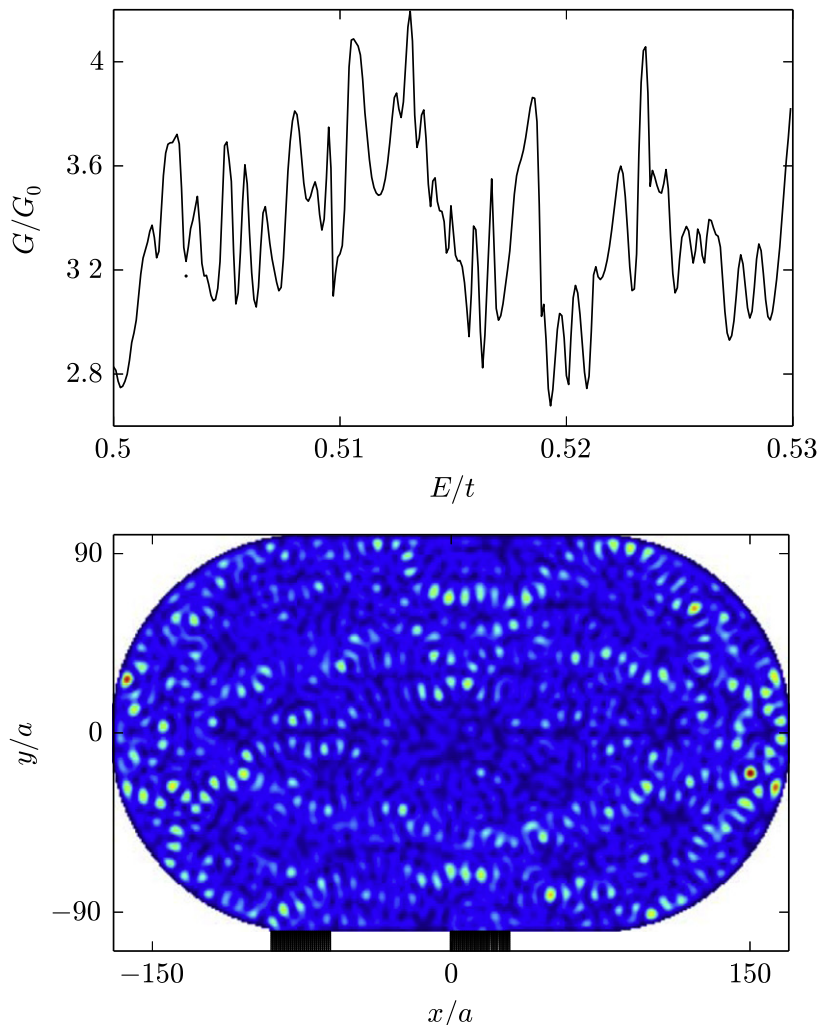
Figure 4. Top panel: dependence of conductance of a stadium billiard on energy showing universal conductance fluctuations. Bottom panel: Color plot of the local density of scattering states in the same billiard at a given energy. The first ten unit cells of the attached semi-infinite lead are visible as a shaded rectangle below the billiard. This figure has been generated by the Kwant script shown in section 5.
