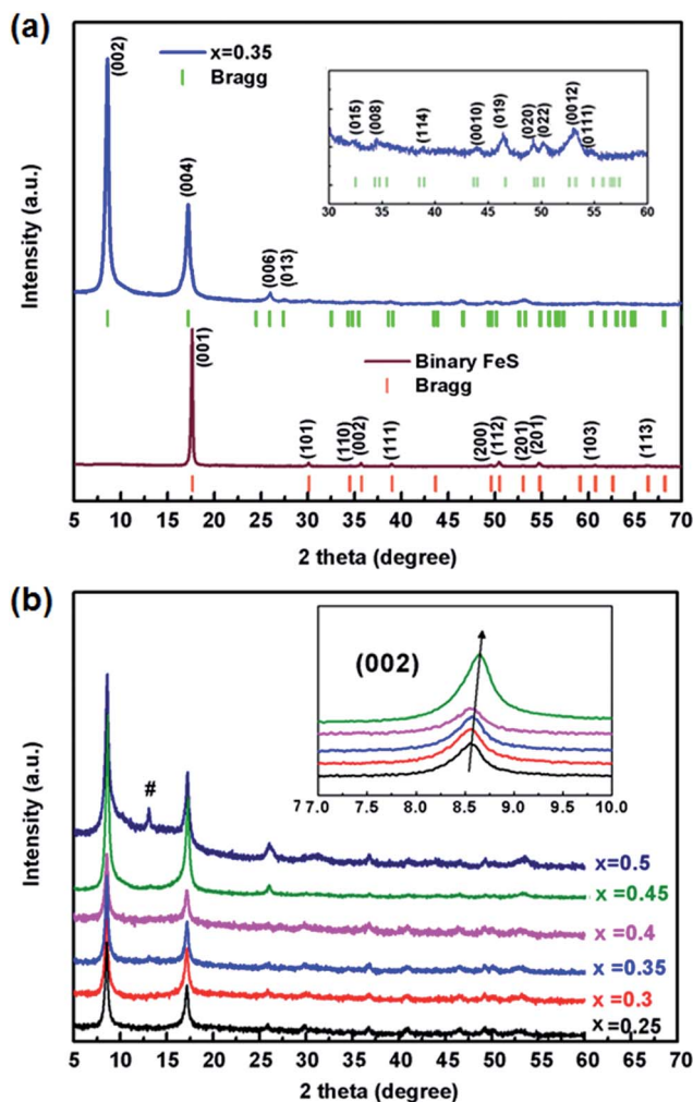
Fig. 1 (a) PXRD pattern of binary FeS and K_x(C_2H_8N_2)_yFe_{2-z}S_2 ( x = 0.35 ), where the green and red vertical lines represent Bragg diffractions of I4/m and P4/nmm space groups, respectively. Inset shows the enlarged pattern of K_x(C_2H_8N_2)_yFe_{2-z}S_2 from 30 to 60 2theta degree. (b) PXRD patterns of K_x(C_2H_8N_2)_yFe_{2-z}S_2 with different x . Inset shows the enlarged (002) peaks. # represents the diffraction peak of 245 phase.
