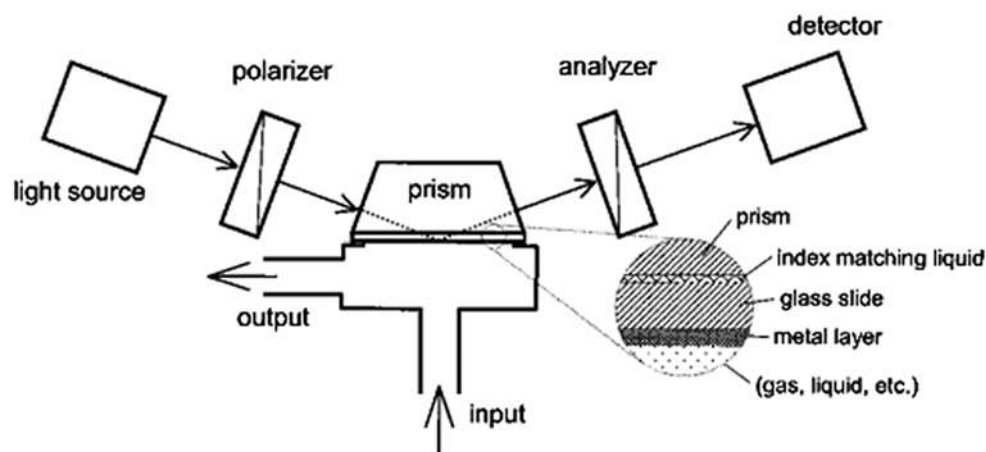
Figure 13: Schematic of TIRE. Magnification shows different stacks of layers between the flow cell and prism. 51
