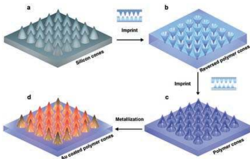
Figure 36: Steps for fabricating 3D cones using nanoimprint lithography; (a) Silicon master; (b) Reverse polymer cones made after imprinting into the polymer layer; (c) Polymer cones made from reversed polymer cones; (d) Gold deposited on top of the cones. 130
