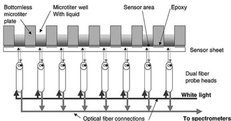
Figure 46: Guided mode resonant filter based biosensors. 166
