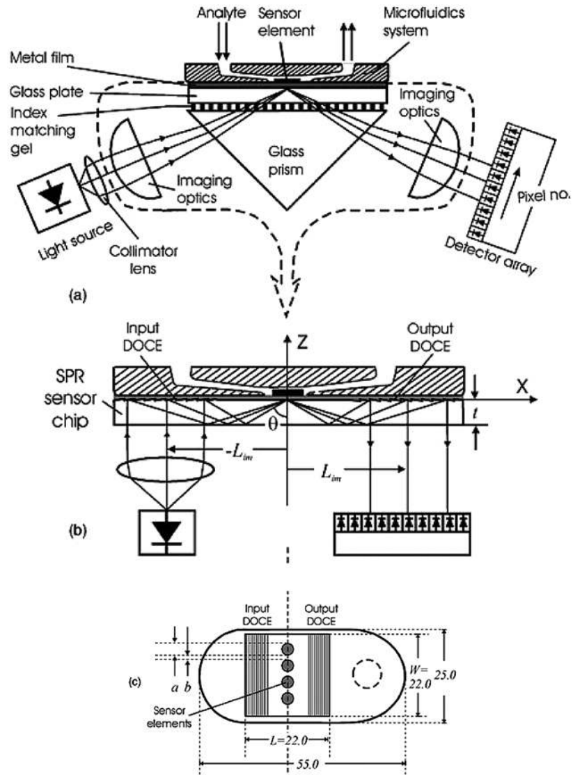
Figure 31: (a) Kretschmann configuration; (b) Modified SPR setup using DOCE; (c) Top view of the polymer chip along with dimensions in mm. 110
