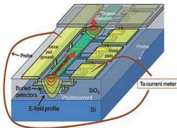
Figure 47: Schematic of LEAC biosensor. 167
