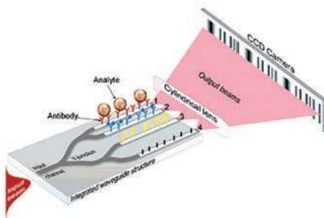
Figure 42: Representation of 4 channel YI showing different antibody immobilization at different channels. 152
