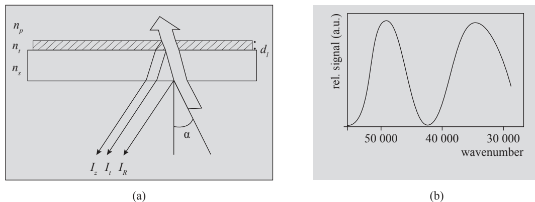
Figure 11: Principle of RIFS sensing (a) Schematic; (b) Corresponding interference pattern. 42
