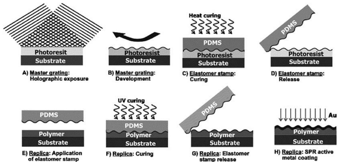
Figure 25: Fabrication steps of diffraction grating. 97
