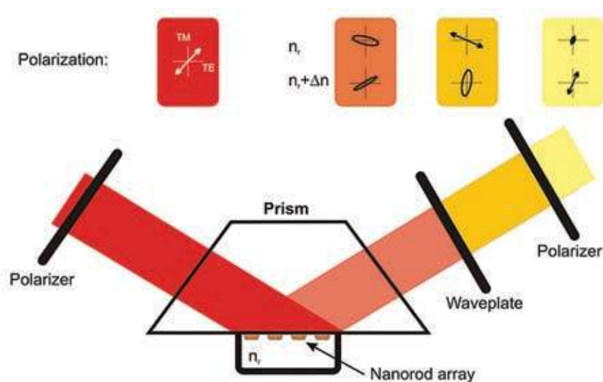
Figure 39: Schematic of an LSPR based optical biosensor using nanorod arrays along with polarization at different positions. 142
