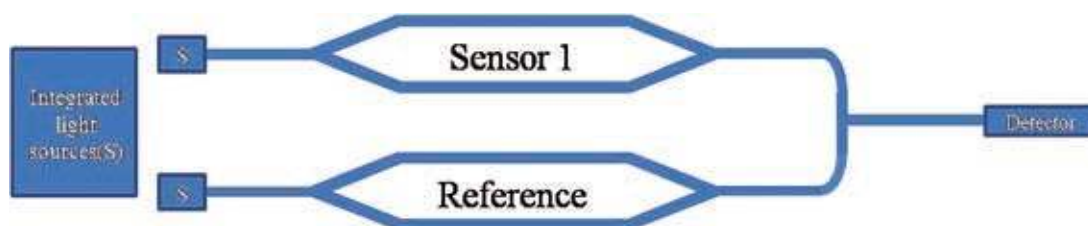
Figure 43: Representation of array of MZI for multiplexing. Adapted from Petrou et al. , 2010.
