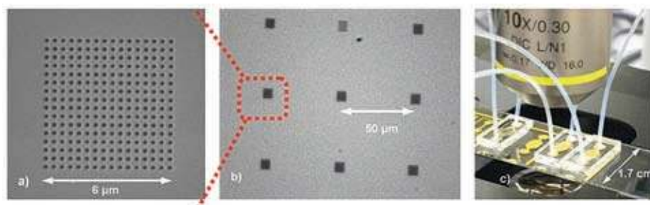
Figure 37: (a) Scanning electron microscopy (SEM) image of a 16 × 16 nanoarray; (b) Bright-field microscope image of a part of 5 × 3 microarray; (c) Microfluidic flow cell along with tubing. 132
