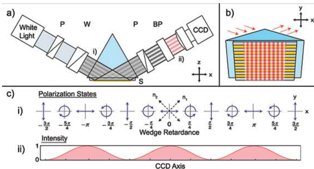
Figure 32: (a) Schematic of SPR-PI showing all the components; (b) Interference Pattern on the sensor surface; (c) Polarization states and Intensity plot. 113
