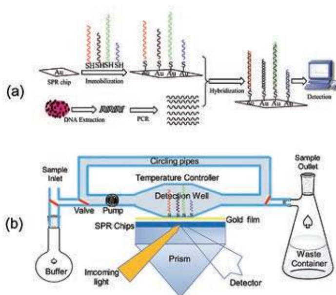
Figure 29: (a) Complete step from immobilization to hybridization and detection; (b) Modified SPR setup. 104
