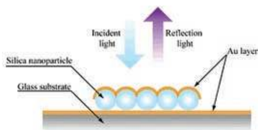
Figure 38: Core shell configuration for LSPR nanochip. 141
