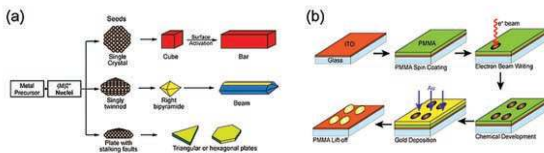
Figure 35: Techniques for fabrication of nano structures; (a) Chemical synthesis; (b) General steps for EBL. 121
