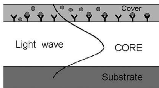
Figure 15: Evanescent field propagating in a waveguide.
