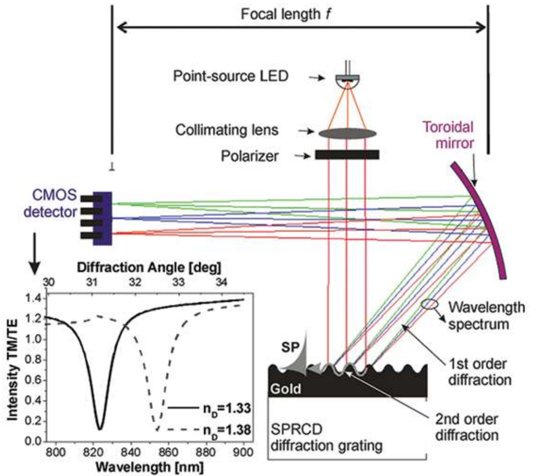
Figure 24: Concept of SPRCD. 94
