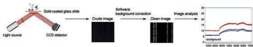
Figure 20: A schematic representation of SPR imaging. 80
