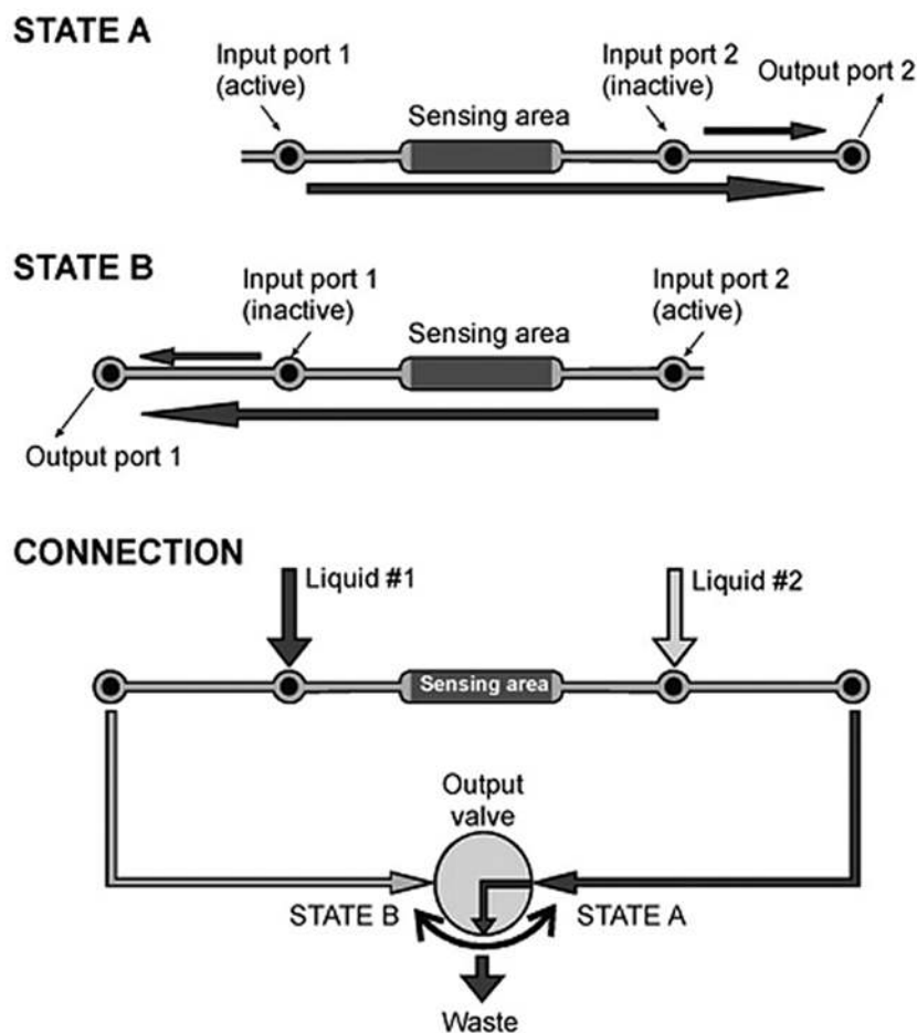
Figure 27: Schematic shows connections of sensing area to ports in different working states. 99
