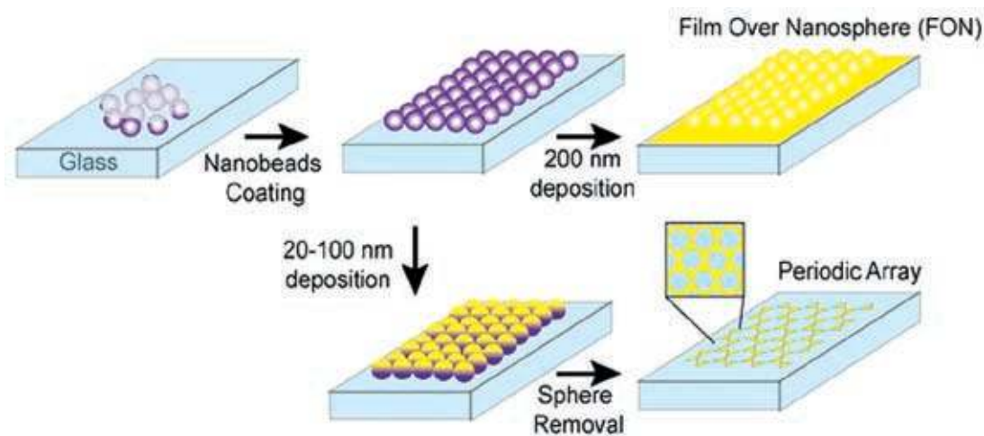
Figure 34: Steps in Nanosphere Lithography (NSL) to fabricate periodic nanoarrays. 121
