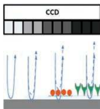
Figure 40: Principle of SRIB: Relative reflectance from different thicknesses can be seen as a change in intensity on CCD. 149
