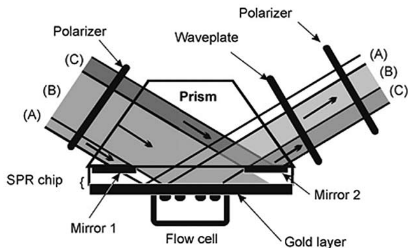
Figure 21: SPR imaging with self-referencing and polarization contrast. Mirror 1 blocks part (A) of incident light and thus the detectors corresponding to that part of the sensor surface provide a reference for the dark current of the detectors since no light is reflected on to the detectors. Mirror 2 reflects part (C) of incident light to the detector for referencing against light source fluctuations. 84
