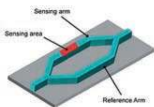
Figure 41: Mach-Zehnder interferometer integrated as waveguide. 41
