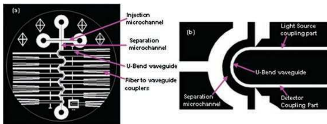
Figure 16: (a) Mask design of the U-bend waveguide; (b) Close-up of a U-bend waveguide. 56
