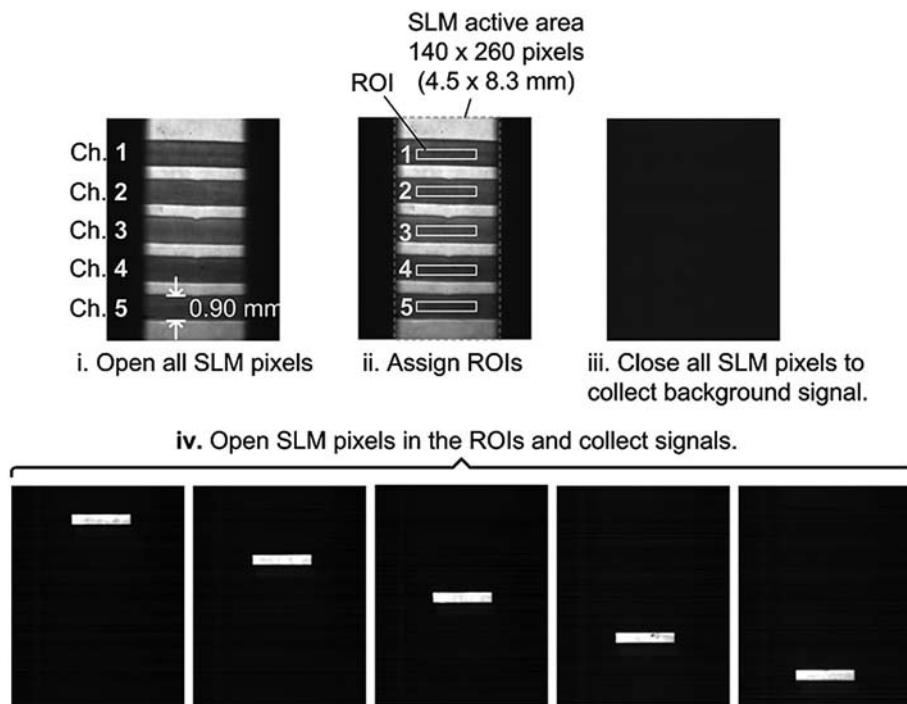
Figure 30: Operating procedures for collecting signal using SLM techniques. 107
