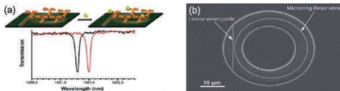
Figure 14: Micro Ring Resonator: (a) Working; (b) Top view of microring with adjacent waveguide. 41
