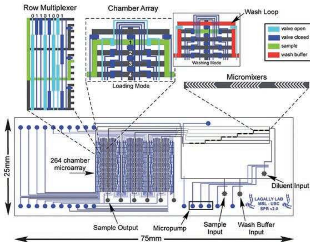
Figure 28: Schematic of microfluidic array. 102
