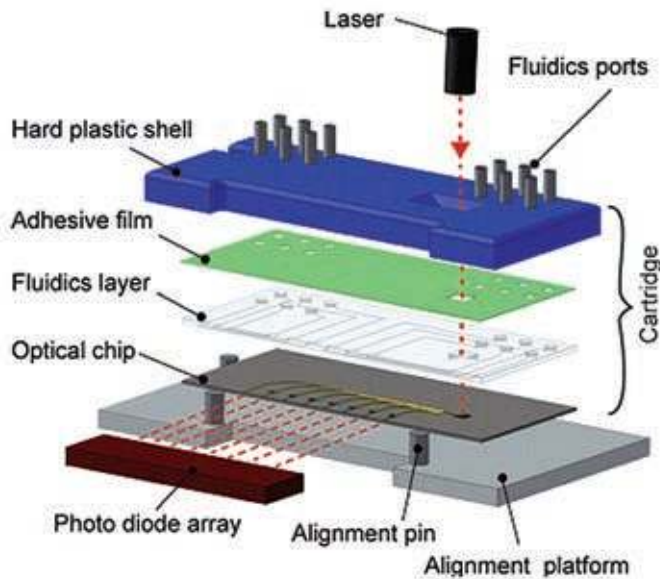
Figure 44: Different parts of the sensing system. At the base is the alignment platform and, above the platform is the optical chip consisting of ring resonators. The optical chip is covered with a hard plastic shell containing the microfluidics channels. 161
