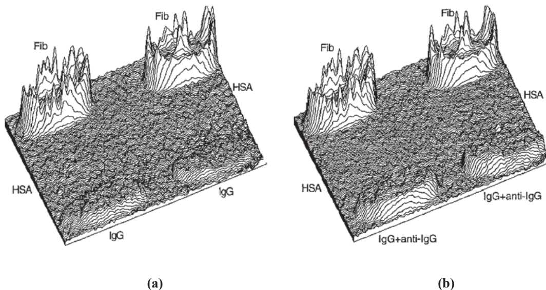
Figure 45: (a) Thickness of the substrate before incubation; (b) Thickness of the substrate after incubation of anti-IgG. 163
