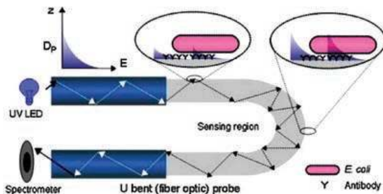
Figure 7: Enhancement of penetration depth ' D_p ' in a bend fiber probe, enabling evanescent field overlap for the detection of E. coli . 32
