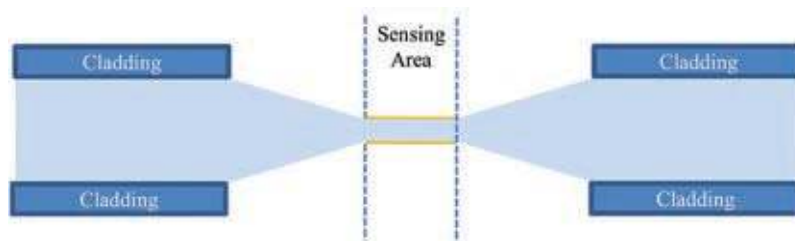
Figure 18: Cross-sectional drawing of a biconical tapered waveguide.
