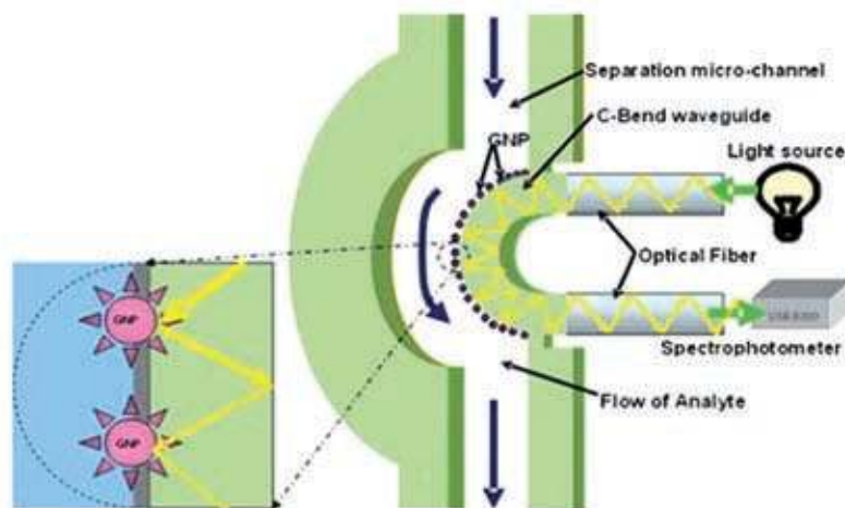
Figure 33: C-bend waveguide coated with GNP for LSPR based detection. The closet on the left shows the generation of surface plasmons due to the interaction of an evanescent wave and GNP. 118
