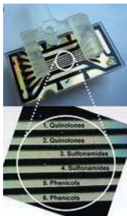
Figure 26: Image of an SPRCD cartridge for detection of antibiotics. 92
