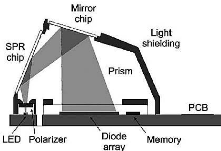
Figure 19: Cross-section of Spreeta 2000, indicating the light path and position of various components. 71
