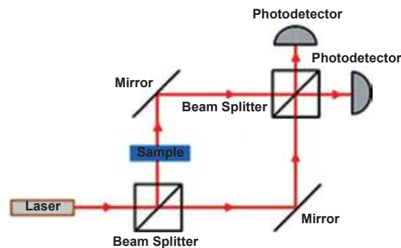
Figure 10: Free space schematic of a Mach-Zehnder interferometer. 41
