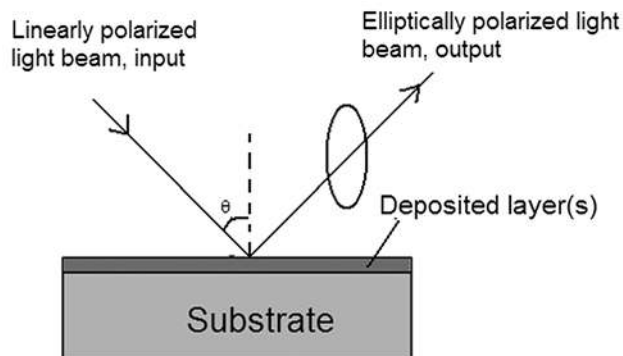
Figure 12: Schematic of principle of measurements using ellipsometry.
