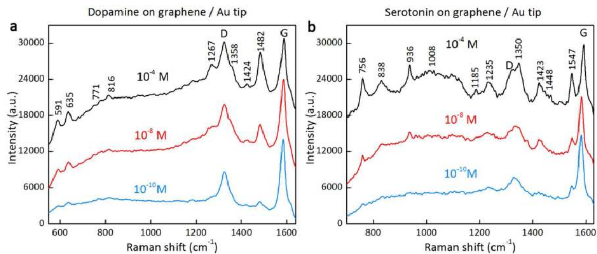
Figure 6. Raman spectra of neurotransmitter molecules on graphene hybrid structure with 3 different concentrations ( 10^{-4} , 10^{-8} , and 10^{-10} M). (a) Dopamine. (b) Serotonin. The laser excitation wavelength is 633 nm.
