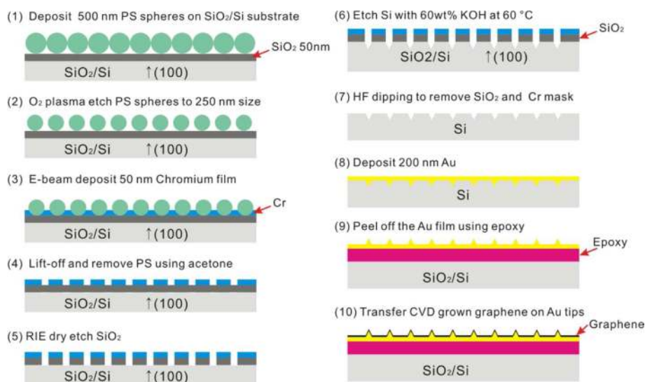
Figure 1. Schematic illustration of the graphene–Au tip hybrid platform fabrication process.
