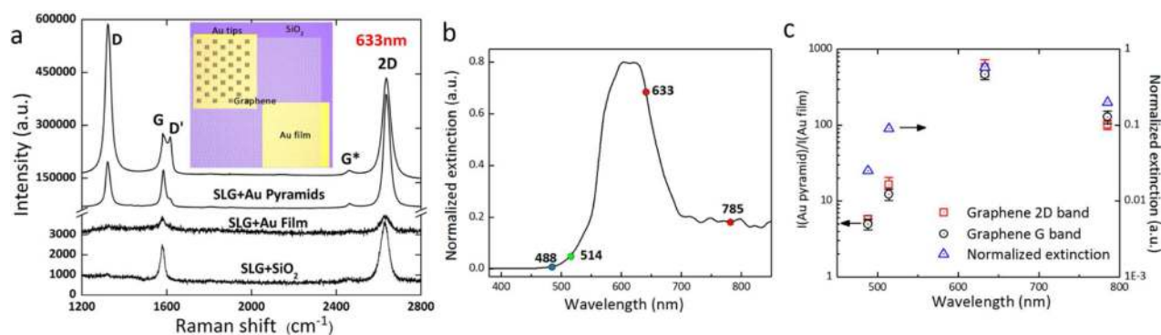
Figure 4. Raman spectra of single layer graphene (SLG) on Au tip structure and the wavelength selectivity. (a) Graphene Raman spectra measured from various surfaces (Au tips, flat Au, and \text{SiO}_2 as shown in the inset) with 633 nm excitation wavelength. (b) The extinction spectrum of Au tips, the three excitation wavelengths of 488, 514, 633, and 785 nm are marked with dots, respectively. (c) Ratios of intensity of graphene G and 2D peaks measured on the Au tip regions to those measured on flat Au regions, as well as normalized extinction at 4 wavelengths. The ratios in semilog scale are plotted as a function of the excitation wavelength.
