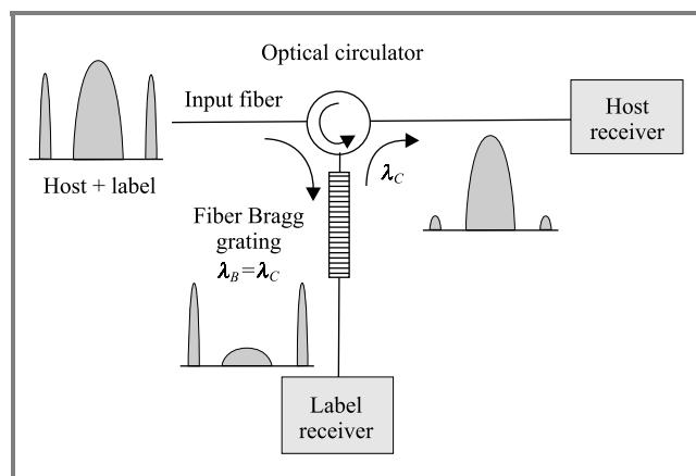
Fig. 11. Separation of host and high frequency label using optical filter [28].
