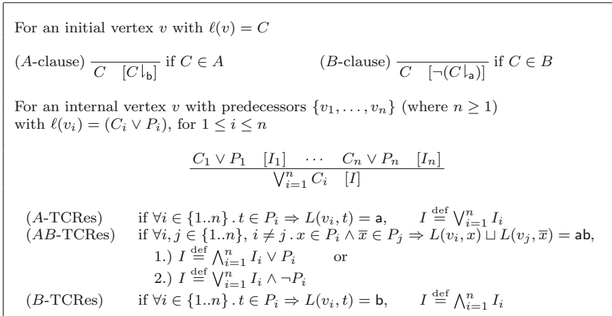
Fig. 6 Labelled interpolation system for clausal proofs
