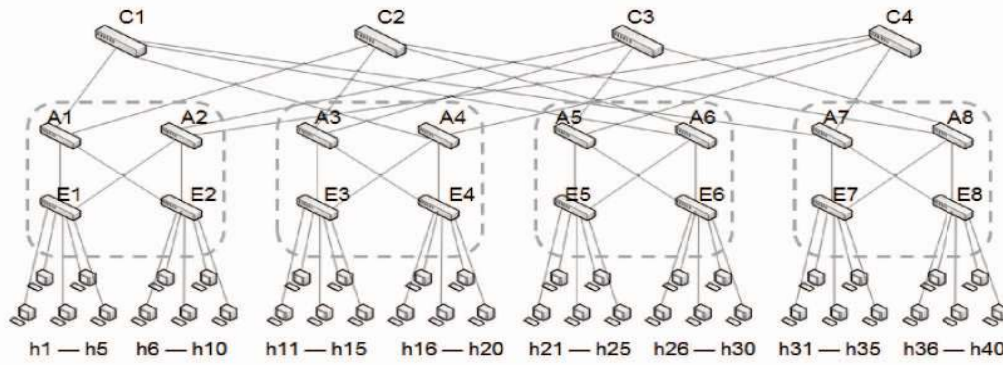
Figure 3. Model B: 3-level fat-tree network topology.
