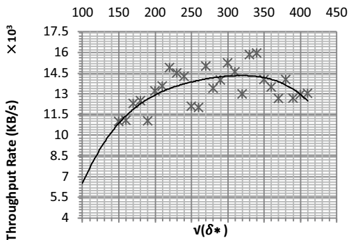
Figure 6. Relationship between one-hop LABERIO trigger and overall throughput.
