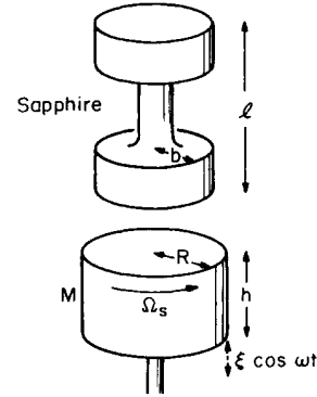
FIG. 6. Experimental configuration for detecting the gravitational analog of Faraday's law of induction.
