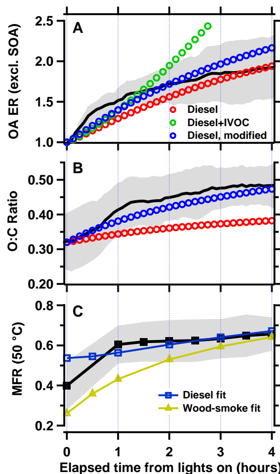
Fig. 7. Time series comparing campaign-average measured and predicted OA: (A) Enhancement ratio corrected for traditional SOA; (B) OA O:C ratio; (C) OA MFR at 50 °C. Black lines indicate average data with grey regions showing \pm one standard deviation. The colors of the lines and symbols are used consistently in all three panels; the symbols indicate model predictions using the different sets of parameters listed in Table 3. Curves in (C) indicate predicted evaporation at equilibrium in the TD using diesel and wood-smoke volatility distributions in the modified aging model. Models based on the wood-smoke and diesel volatility distributions have nearly identical predicted OA ER and O:C time series.
