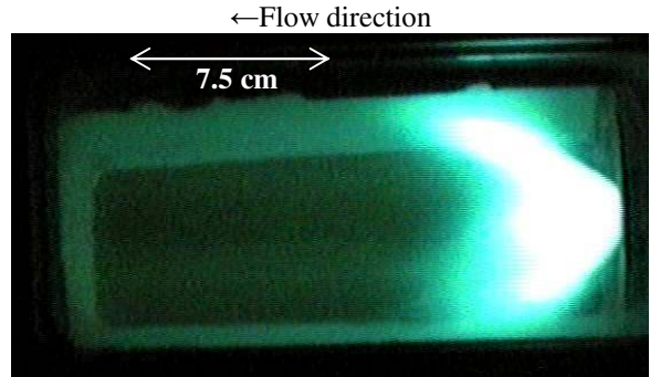
(a) 8% \text{H}_2 61% \text{CO} 31% \text{CH}_4 \phi = 0.55 T = 444\text{K} and P = 7.9\text{atm} , U_0 = 17.0 \text{ m/s}
