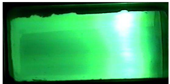
(c) 15% \text{H}_2 68% \text{CO} 17% \text{CH}_4 \phi = 0.41 T = 442\text{K} and P = 7.87 \text{ atm} , U_0 = 16.87 \text{ m/s}
