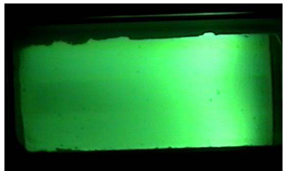
(d) 51% \text{H}_2 26% \text{CO} 23% \text{CH}_4 . \phi = 0.39 T = 442\text{K} and P = 7.87\text{atm} , U_0 = 16.65 \text{ m/s} ,
