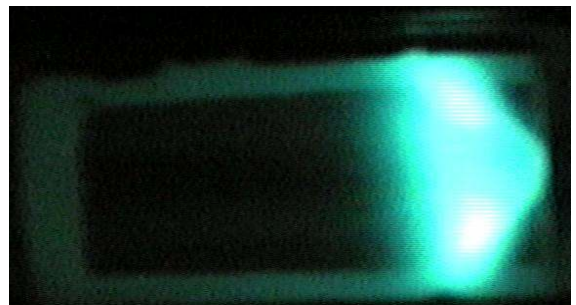
(b) 20% \text{H}_2 40% \text{CO} 40% \text{CH}_4 \phi = 0.28 T = 509 \text{ K} and P = 7.8\text{atm} , U_0 = 31.8 \text{ m/s} ,
