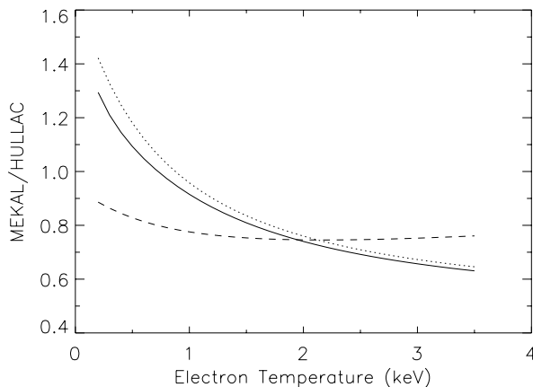
FIG. 6.—Comparison between the HULLAC rate coefficients and MEKAL model. The solid line is for the 3p_{3/2} \rightarrow 2s_{1/2} transition, the dotted line is for the 3p_{1/2} \rightarrow 2s_{1/2} transition, and the dashed line is for the 3d_{5/2} \rightarrow 2p_{3/2} transition.
