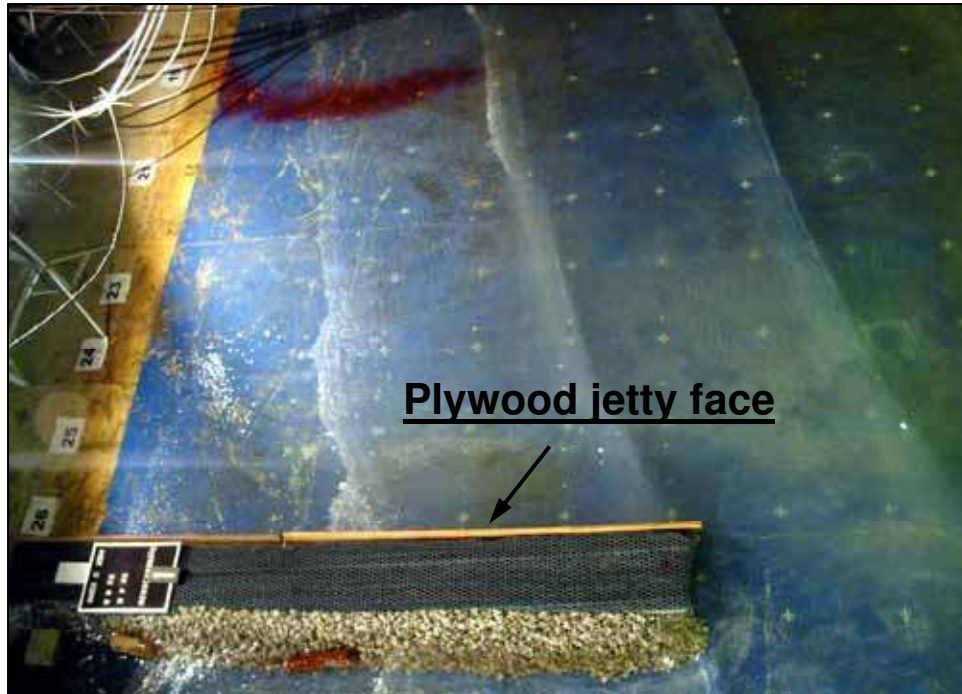
Figure 10. Plywood reflecting jetty face
