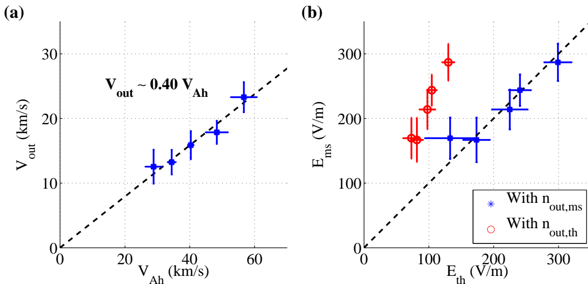
FIG. 5. (color online) (a) Measured ion outflow velocity compared to the hybrid Alfvén velocity. The measured values are about 40% of theoretically predicted values. The black dashed line indicates a linear fit. (b) The measured reconnection electric field versus E_{th} in Eqn. 3. Values of E_{ms} agree with those of E_{th} when the measured outflow density, n_{out,ms} (blue asterisks) is used as n_{out} instead of the theoretical estimate, n_{out,th} (red circles).
