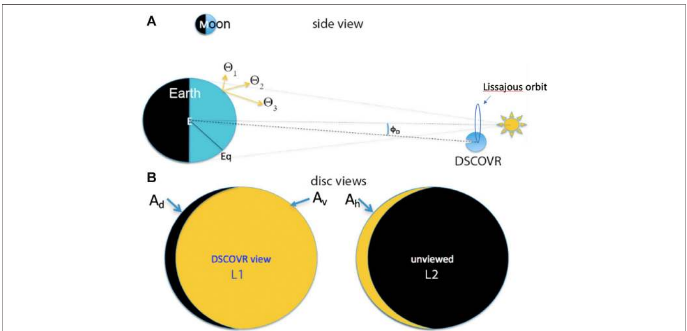
FIGURE 3 | Schematic of (A) Earth-Sun-DSCOVR geometry and (B) portion of sunlit Earth disc viewed by DSCOVR and the portion that would be viewed at L2 (right). Golden area on left is the daytime area fraction, A_v , visible to DSCOVR and the black area, A_d , is the nighttime fraction seen by DSCOVR. The dark fraction is enhanced for purposes of illustration. The golden area on the right indicates the sunlit fraction, A_h , not seen by DSCOVR. Not to scale. (Adapted from Su et al., 2018).
