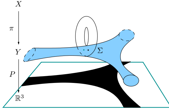
Figure 6: Negative fibration with amoeba-like discriminant.
