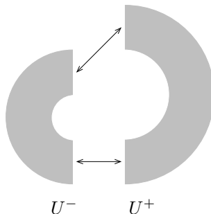
Figure 10: Gluing half annuli with different radii.
