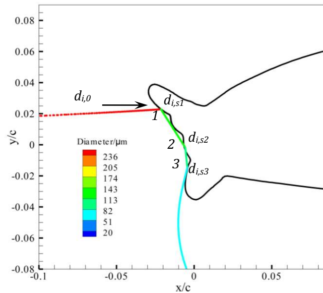
Fig. 7 The splashed droplet trajectory (MVD=236 \mu m)
