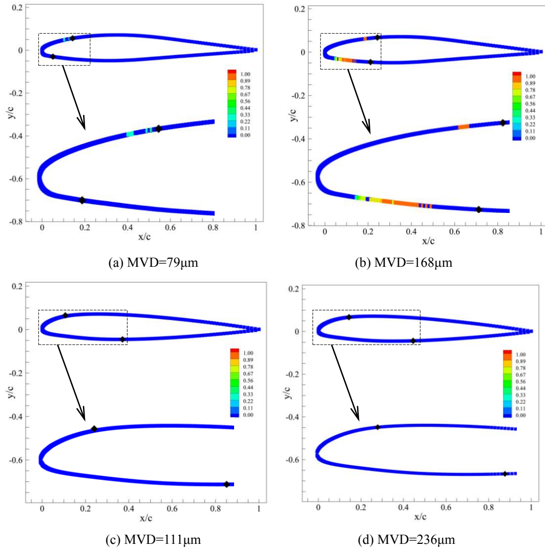
Fig. 14 Mass back ratio distributions on the clean surfaces of the twin-otter [(a) and (b)] and the NACA23012 [(c) and (d)] airfoils
