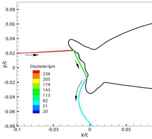
(b) splashing occurs, n=2
