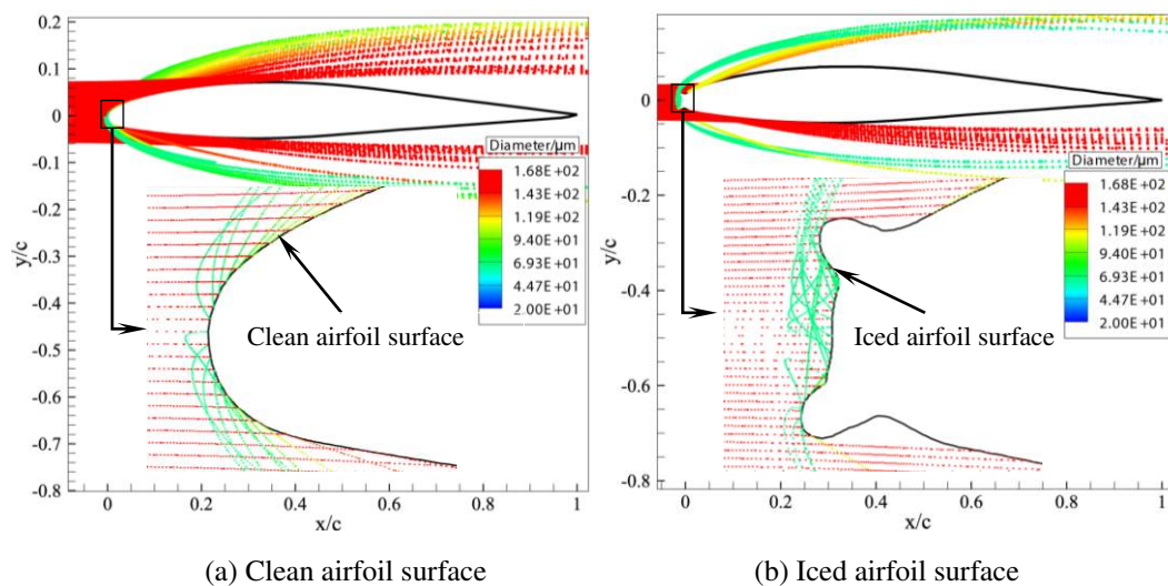
Fig. 11 Droplet splashing and re-impingement on the clean (left) and iced (right) Twin Otter airfoil surface at MVD=168 \mu m
