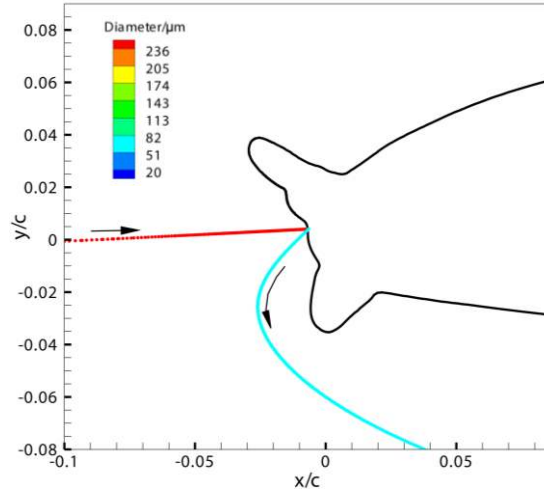
(a) Splashing occurs, n=1
