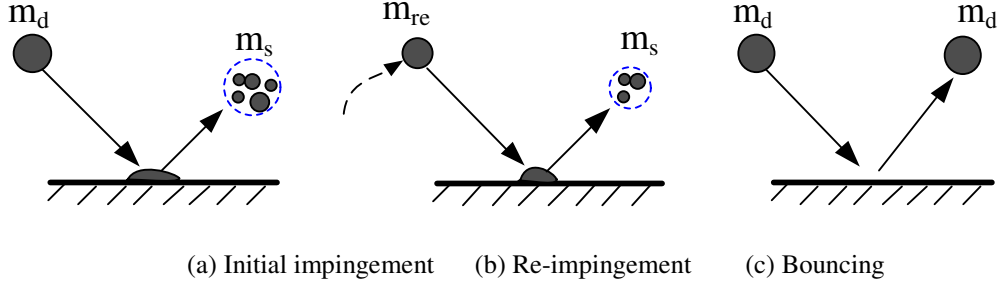
Fig. 3 Droplet-wall interaction with droplet splashing and bouncing
