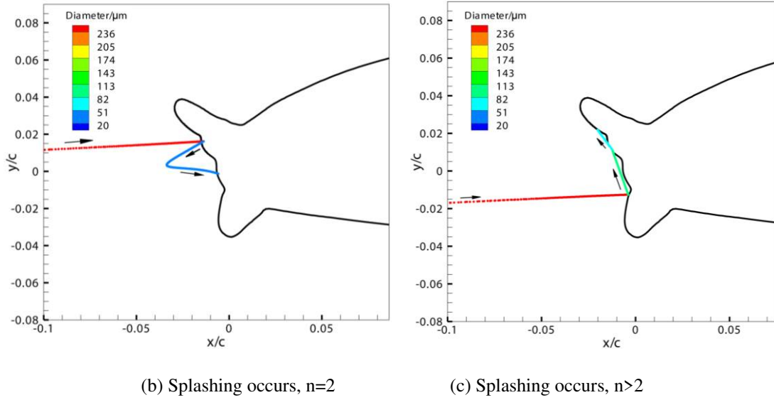
Fig. 5 Droplet trajectory with the TP on the solid surface (MVD=236 \mu\text{m} )
