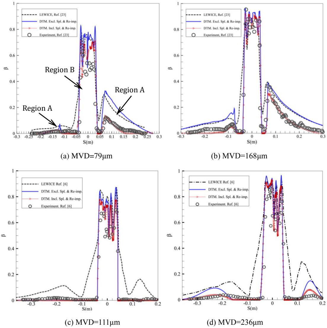
Fig. 10 SLD impingement distributions on the iced airfoil surfaces of the Twin Otter [(a) and (b)] and the NACA23012 [(c) and (d)]
