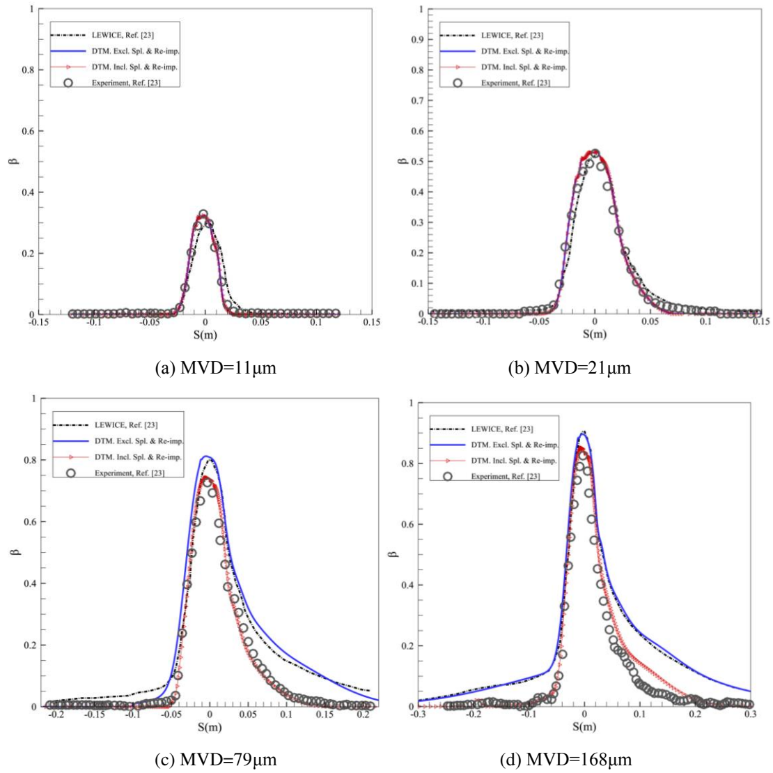
Fig. 8 Comparison of \beta distribution between computational and experimental results on the clean Twin-Otter airfoil surface
