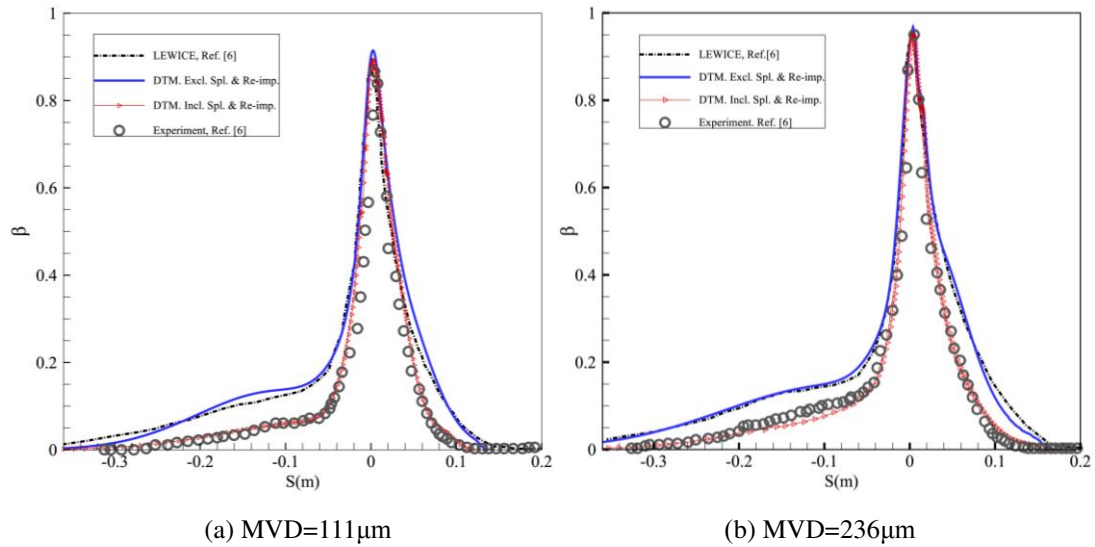
Fig. 9 Comparison of \beta distribution between the numerical and experimental results on the clean NACA23012 airfoil surface
