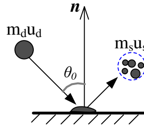
Fig. 4 Mass and momentum change due to droplet splashing.
