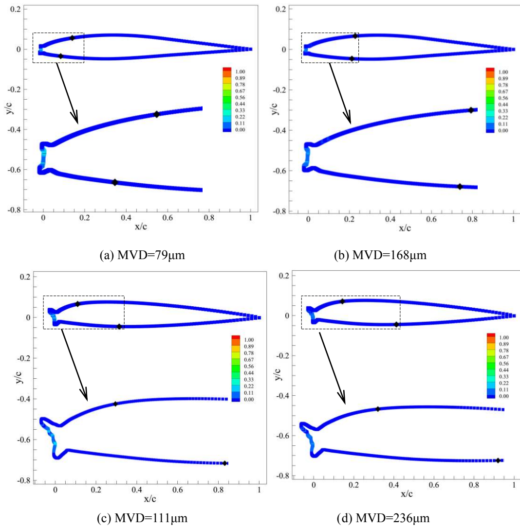
Fig. 15 Mass back ratio distributions on the “iced” surfaces of the twin-otter [(a) and (b)] and the NACA23012 [(c) and (d)] airfoils
