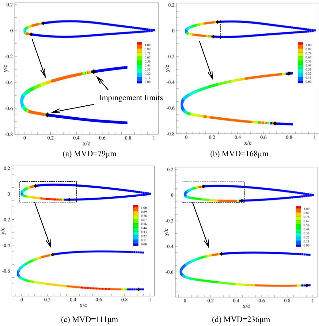
Fig. 12 Mass loss ratio distributions on the clean airfoil surfaces of the twin-otter [(a) and (b)] and the NACA23012 [(c) and (d)]
