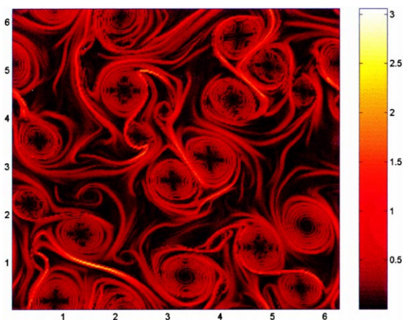
Fig. 16. The relative dispersion density field d^2(t, \mathbf{x}_0) at t = 10 . (We actually plot \sqrt{d^2(t, \mathbf{x}_0)} for better visibility of the structures.)
