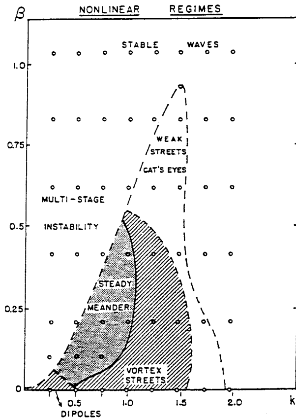
FIG. 3. Nonlinear regime diagram from Flierl et al. (1987) identifying different types of finite-amplitude flow evolution in (\beta, k_0) phase space for the nonlinear barotropic numerical model.
