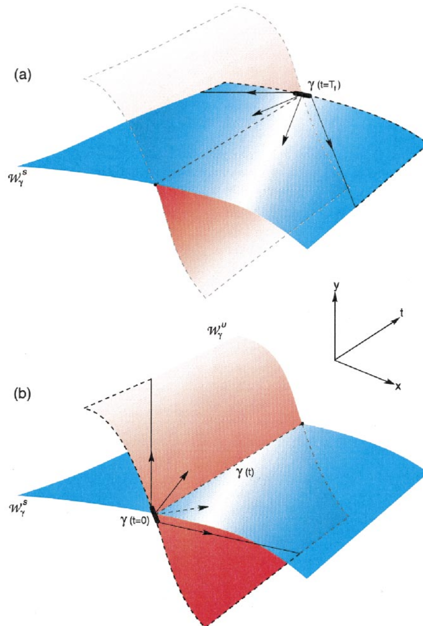
FIG. 7. Schematic of the computational approach used to approximate the finite-time material surfaces and the hyperbolic trajectory \gamma(t) . (a) The stable surface, \mathcal{W}_\gamma^s (shown in blue), is generated by trajectories that exponentially move away from the hyperbolic region in the vicinity of \gamma(t = T_f) as time regresses; (b) the unstable surface, \mathcal{W}_\gamma^u (shown in red), is generated by trajectories that exponentially move away from \gamma(t = 0) as time progresses. Portions of \mathcal{W}_\gamma^s [in (a)] and \mathcal{W}_\gamma^u [in (b)] outlined with the dotted line are not computed but are included in the figure to aid the visualization of the surfaces.
