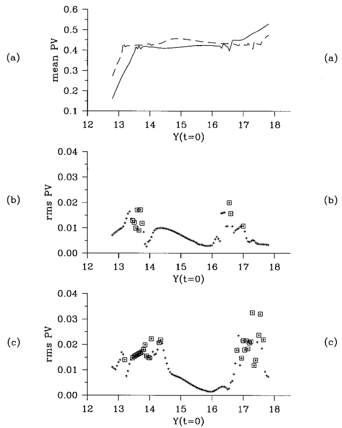
FIG. 15. Lagrangian potential vorticity statistics for case III. (a) Mean potential vorticity vs initial meridional location, Y(t = 0) , for the western transect (plotted with the solid line) and eastern transect (plotted with the dashed line) shown in Fig. 13b. (b) Standard deviation vs initial meridional location for the western transect. Particle trajectories that exhibit rapid potential vorticity transitions ( \Delta q > 0.015 over 10 time units) have their rms data point augmented with a square. (c) As in (b) but for the eastern transect.
