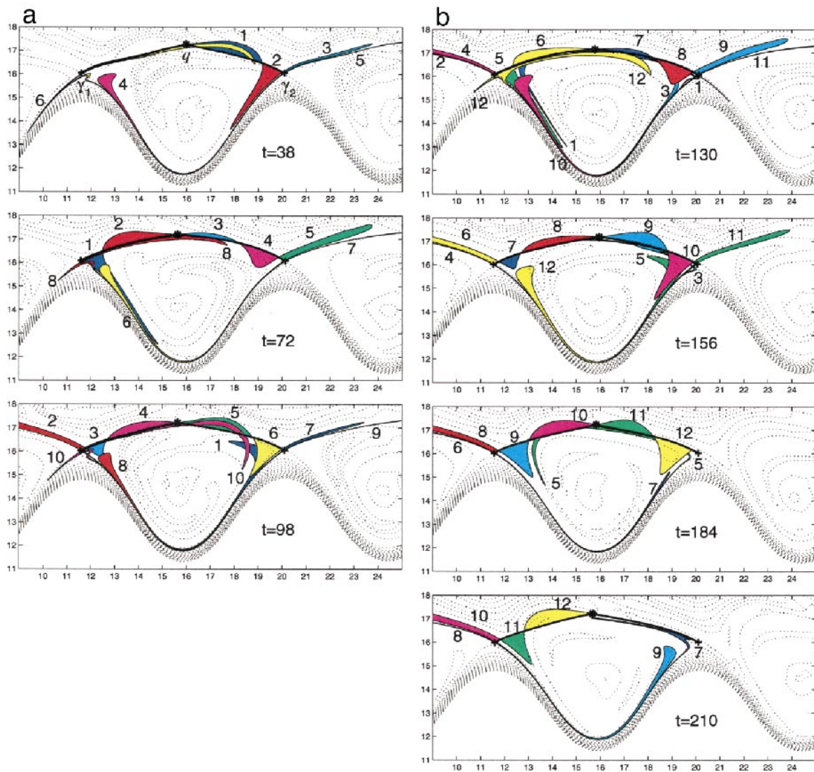
FIG. 9. Results of the aperiodic analysis for case I corresponding to (\text{Re}, \beta, k_0) = (10^4, 0.103, 0.74) .
