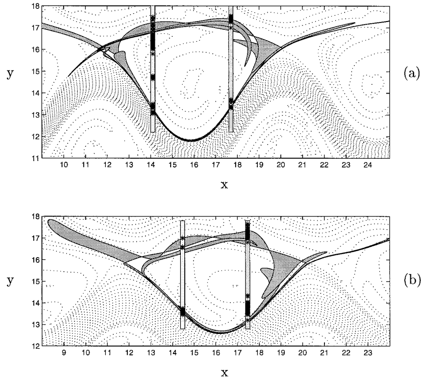
FIG. 13. Composite illustrations of the potential vorticity field (contoured in the dotted line style), lobe structure (shaded), and two meridional transects through the cat's eye region where Lagrangian particles are initially positioned 0.05 units apart for (a) case I at time t = 98 , and (b) case III at time t = 102 . A total of 242 [202] particles for (a) [(b)] are tracked for 200 time units. The initial positions of particles that exhibit rapid potential vorticity transitions, \Delta q > 0.01 [ \Delta q > 0.015 ] for (a) [(b)] over any 10-unit time interval, are plotted with an asterisk (see also Figs. 14 and 15).
