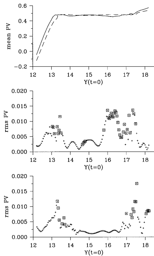
FIG. 14. Lagrangian potential vorticity statistics for case I. (a) Mean potential vorticity vs initial meridional location, Y(t = 0) , for the western transect (plotted with the solid line) and eastern transect (plotted with the dashed line) shown in Fig. 13a. (b) Standard deviation vs initial meridional location for the western transect. Particle trajectories that exhibit rapid potential vorticity transitions ( \Delta q > 0.01 over 10 time units) have their rms data point augmented with a square. (c) As in (b) but for the eastern transect.
