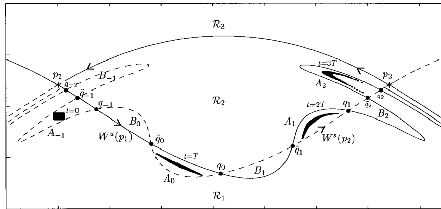
FIG. 2. Poincaré map for the time-periodic meandering jet flow analyzed by Pratt et al. (1995), from Miller et al. (1996), illustrating the chaotic transport between regions \mathcal{R}_1 and \mathcal{R}_2 . Two hyperbolic points, p_1 and p_2 , are indicated. Intersections of the stable manifold W^s(p_2) (dashed line) and unstable manifold W^u(p_1) (solid line) define primary intersection points, q_n and \tilde{q}_n , and lobes A_n and B_n . The regime boundary is defined in this case as W^u(p_1, q_0) \cup W^s(q_0, p_2) . The mapping of a square patch of fluid within lobe A_{-1} to lobes A_0 , A_1 , and A_2 at subsequent times is illustrated.
