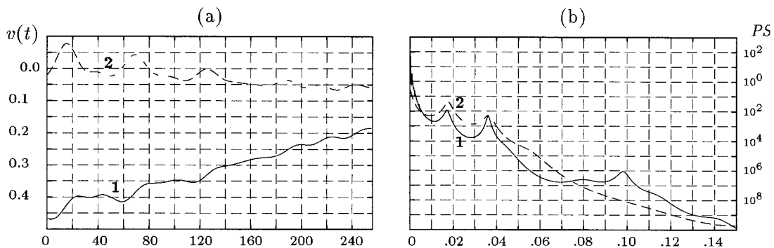
FIG. 6. Time dependence of the flow in the moving reference frame for case III. (a) Time series of the meridional velocity, v(t) , in the moving reference frame for a point located near the jet axis at (x, y) = (6.0, 12.8) (marked "1"), and for a point located in a recirculation region at (x, y) = (8.0, 15.0) (marked "2"). (b) The corresponding power spectrum. The spectral peaks in the range \omega/(2\pi) = (0.017, 0.018) are associated with the nutation period.
