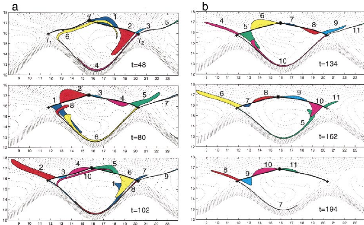
FIG. 11. Results of the aperiodic analysis for case III corresponding to (\text{Re}, \beta, k_0) = (10^3, 0.103, 0.74) .
