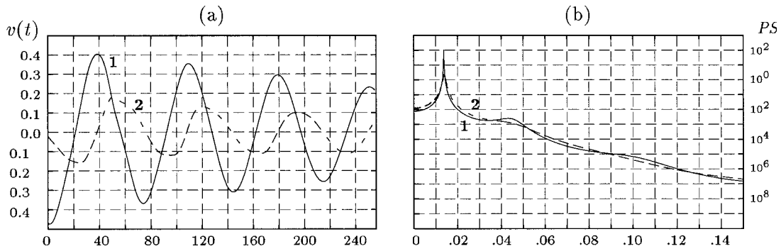
FIG. 5. Time dependence of the flow in the stationary reference frame for case III. (a) Time series of the meridional velocity, v(t) , in the stationary reference frame for two points, located at (x, y) = (6.0, 12.8) (marked "1") and (x, y) = (8.0, 15.0) (marked "2"). (b) The power spectrum obtained using the maximum entropy method. The spectral peak at \omega/(2\pi) = 0.0138 corresponds to the propagation speed of the dominant meander, c = (L_D/n_0) (\omega/(2\pi)) .
