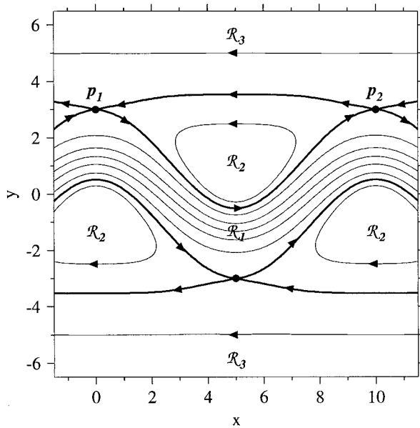
FIG. 1. Streamfunction contours in the moving reference frame for the kinematic model of the meandering jet from Bower (1991). The bounding streamlines separating the prograde ( \mathcal{R}_1 ), recirculation ( \mathcal{R}_2 ), and retrograde ( \mathcal{R}_3 ) regions are drawn with thick lines. Two hyperbolic points, p_1 and p_2 , are indicated.
