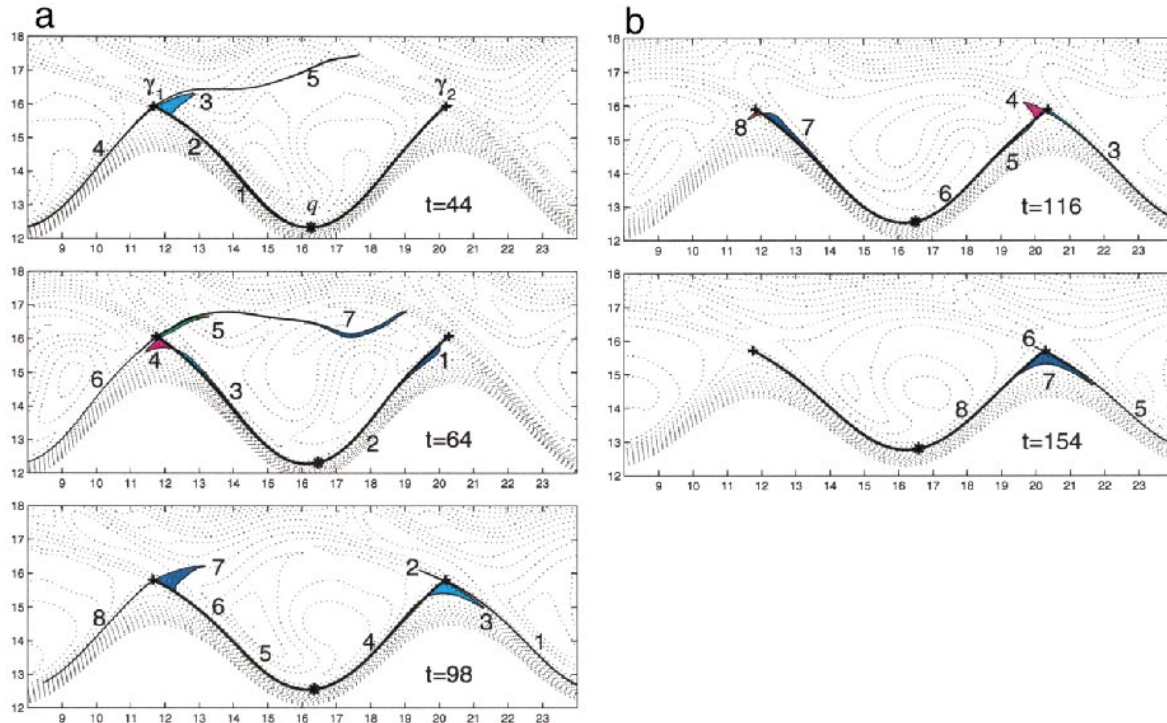
FIG. 12. Results of the aperiodic analysis depicting the jet core-recirculation exchange for case III.
