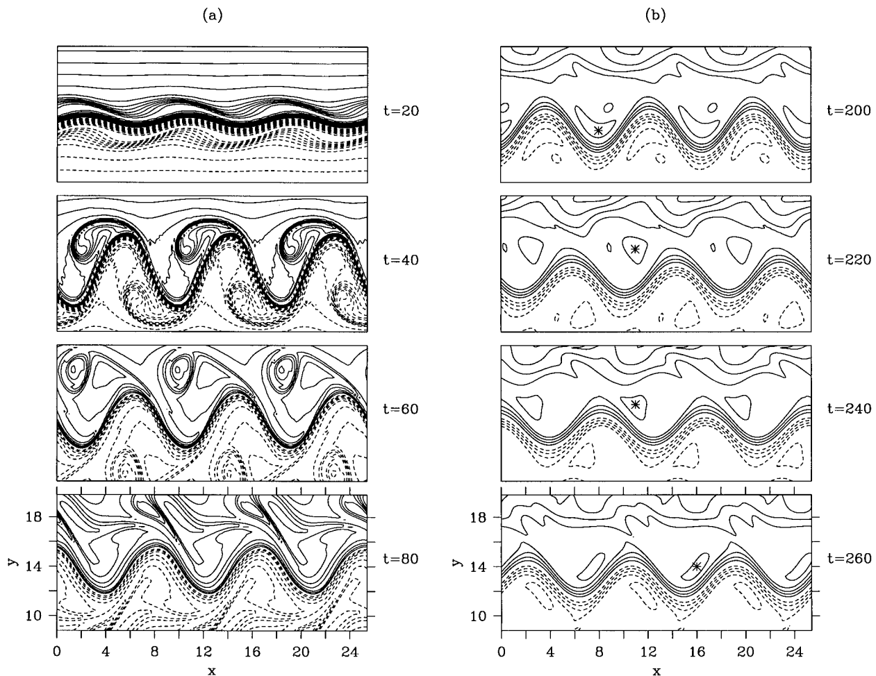
FIG. 4. Evolution of the numerically generated flow as represented by the potential vorticity field for case III. The contour increment is \Delta q = 0.1 . Only a portion of the computational domain is shown. (a) The early nonlinear evolution of the unstable jet, t = 20, 40, 60, 80 . (b) The nearly time-periodic meandering jet flow, t = 200, 220, 240, 260 . A patch of vorticity within a recirculation region is marked with an asterisk.
