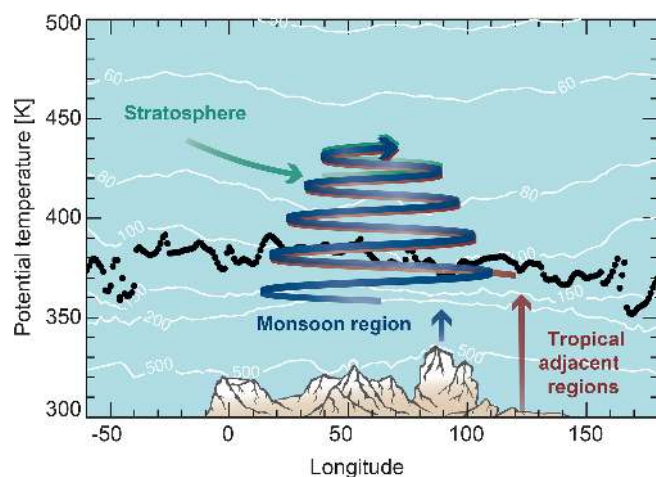
Figure 15. Longitude–theta cross section at about 30^\circ N. At the top of the Asian monsoon anticyclone (above \sim 360 K) air masses circulate around the anticyclone in a large-scale upward spiral extending from northern Africa to the western Pacific. In the upward spiralling range air masses from inside the Asian monsoon anticyclone (shown in blue) are mixed with air masses convectively uplifted outside the core of the Asian monsoon anticyclone in the tropical adjacent regions, e.g. uplifted by tropical cyclones in the western Pacific ocean (shown in red). The higher the air masses are above the thermal tropopause, the larger the contribution of air masses is from outside the Asian monsoon anticyclone from the stratospheric background coming into the upward spiralling flow (shown in green). The levels of pressure are marked by thin white lines and the thermal tropopause is shown by black dots.
