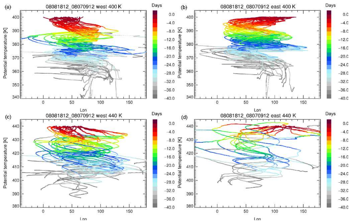
Figure 7. Potential temperature of different 40-day backward trajectories started at 400 K ( a, b ) and 440 K ( c, d ) in the western ( a, c ) and eastern ( b, d ) mode of the Asian monsoon anticyclone are shown versus longitude, colour-coded by days back from 18 August 2008.
