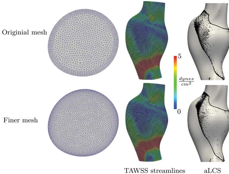
FIGURE 7. Comparison of the TAWSS streamlines and attracting LCS (aLCS) obtained from the original mesh (next to wall edge size 200 \mu\text{m} ) to a finer mesh (next to wall edge size 100 \mu\text{m} ) in the first patient. The TAWSS streamlines are colored based on the TAWSS vector magnitude.
