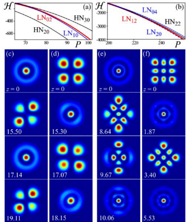
FIG. 4 (color online). (a,b) Energy crossings chosen from the overlapping of two (\mathcal{H}, P) diagrams in Figs. 2(a) and 2(b). Examples of the propagation dynamics of (c) \text{LN}_{10} soliton with P = 100 , (d) \text{HN}_{11} (quadrupole, same as \text{LN}_{02} ) with P = 75 , (e) \text{LN}_{20} with P = 250 , and (f) \text{HN}_{22} with P = 210 .
