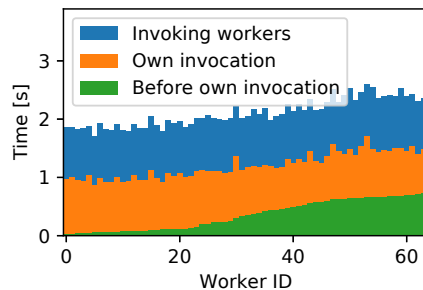
Figure 3: Example run of two-level invocation process.
