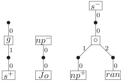
Figure 4: AB lexicon
