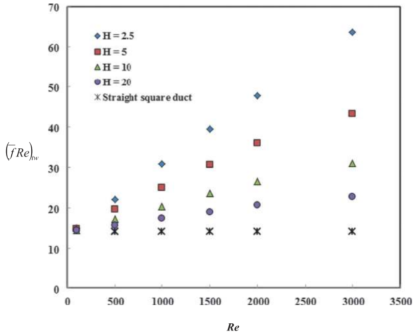
Figure 2. Numerical friction factors for the laminar flow regime.
