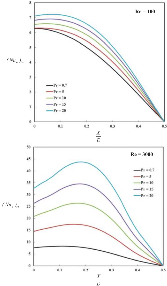
Figure 13. Local heat transfer solution at wall (cb) for H = 20 .
