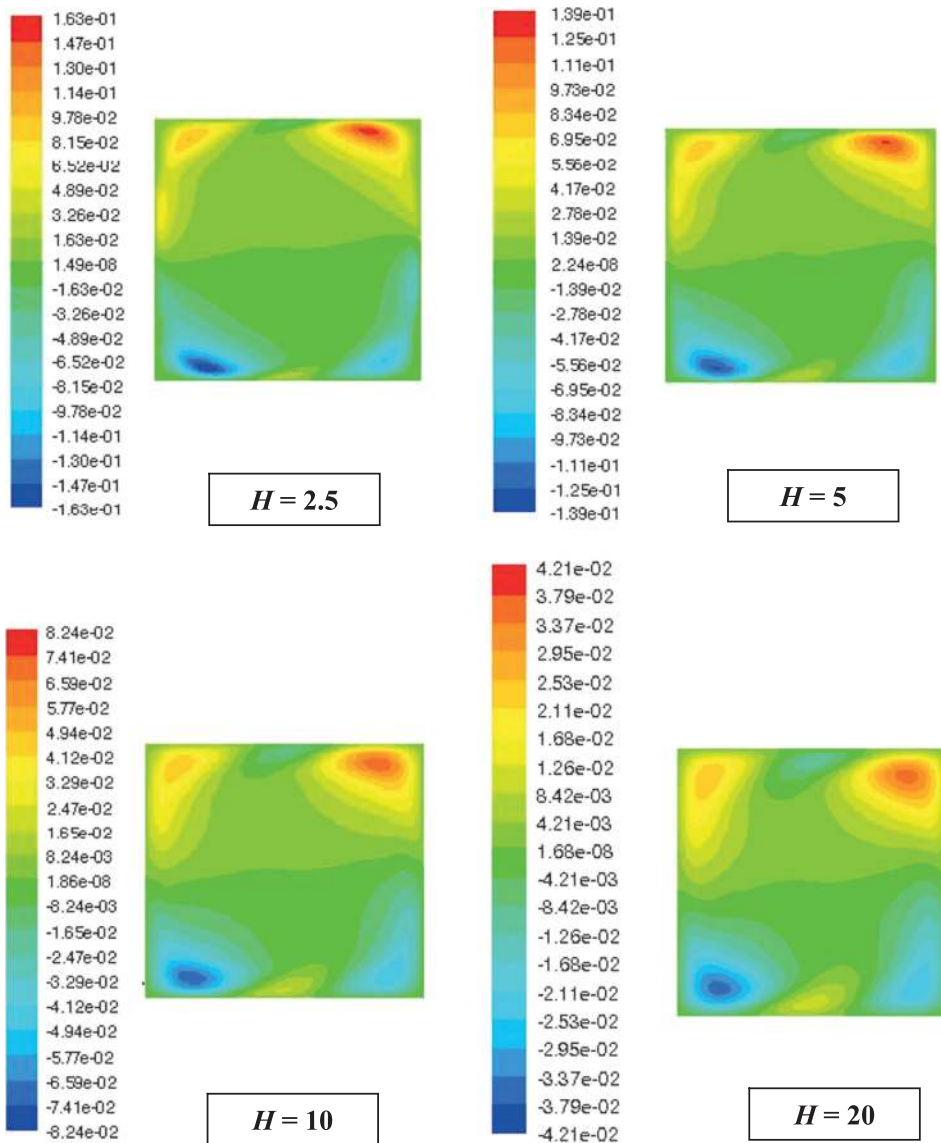
Figure 8. Contours of non-dimensional x velocity ( V_x/V_{mi} ) for a different twist ratio at Re = 100 .
