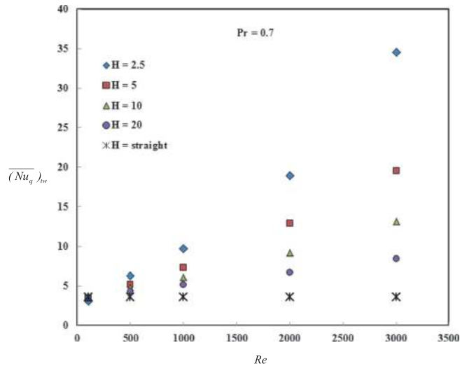
Figure 5. Heat transfer solution for Pr = 0.7 .
