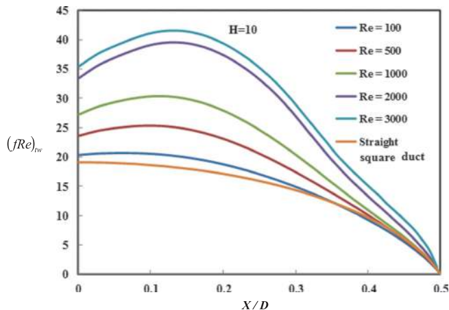
Figure 7. Variation of local fRe along the wall ( cb ) for H = 10 .
