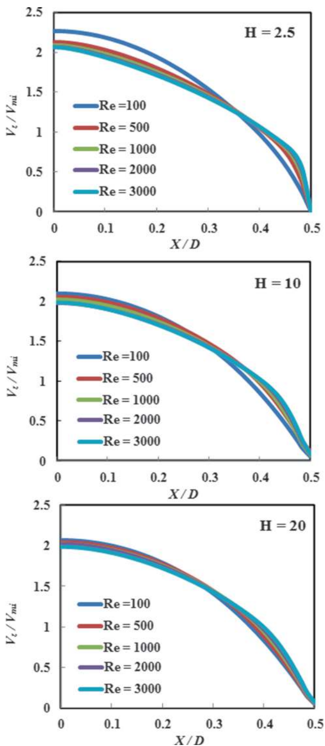
Figure 10. Effect of twist ratio on velocity in the direction of flow.
