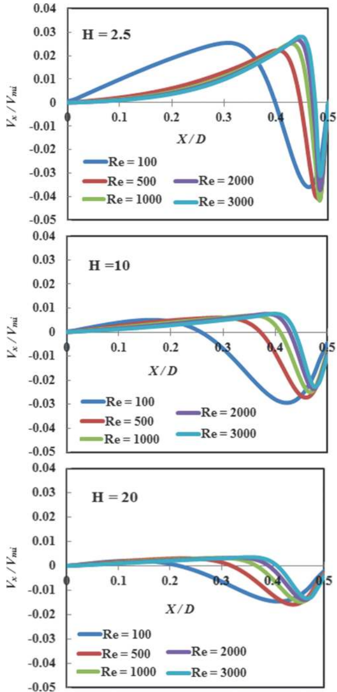
Figure 9. Effect of twist ratio on secondary flow (line ob).
