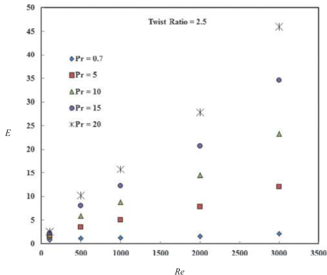
Figure 14. Suitability of twisted square duct for different fluids ( H = 2.5 ).
