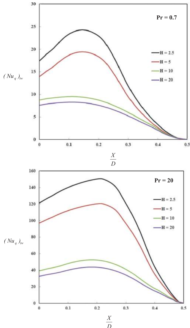
Figure 11. Effect of twist ratio on heat transfer along wall ( cb ) for Re = 3000 .
