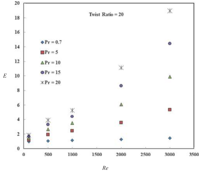
Figure 15. Suitability of twisted square duct for different fluids ( H = 20 ).
