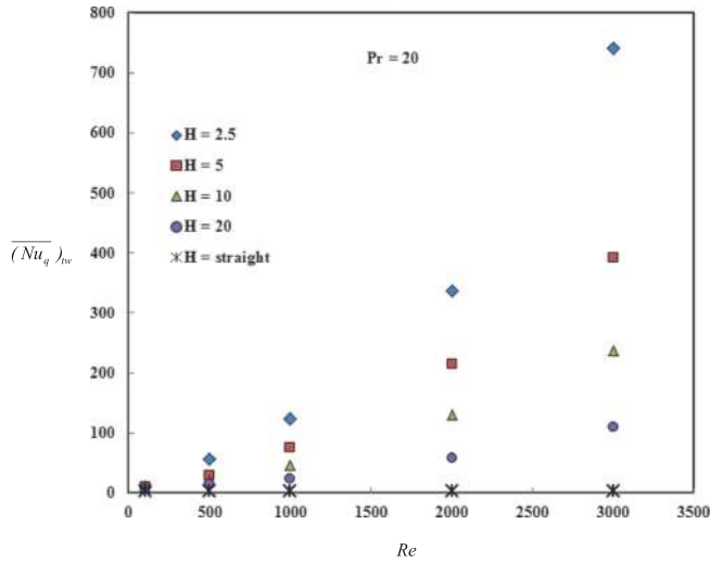
Figure 6. Heat transfer solution for Pr = 20 .
