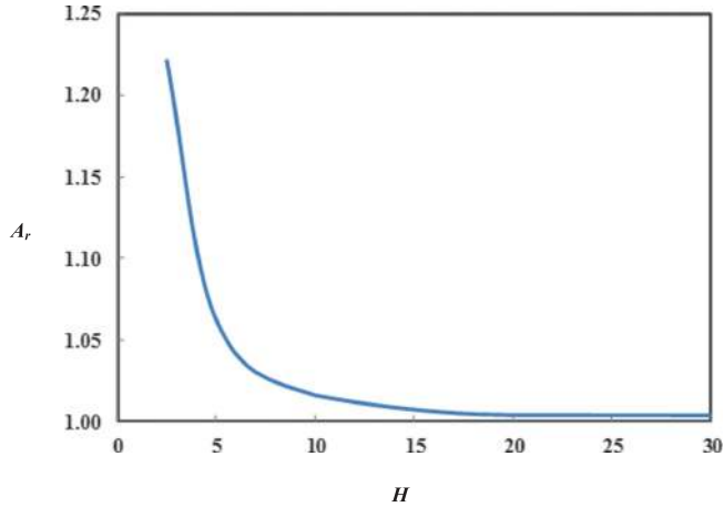
Figure 3. Effect of twist ratio on heat transfer area.
