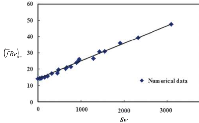
Figure 4. Variations of average friction factor with swirl parameter (Laminar flow).
