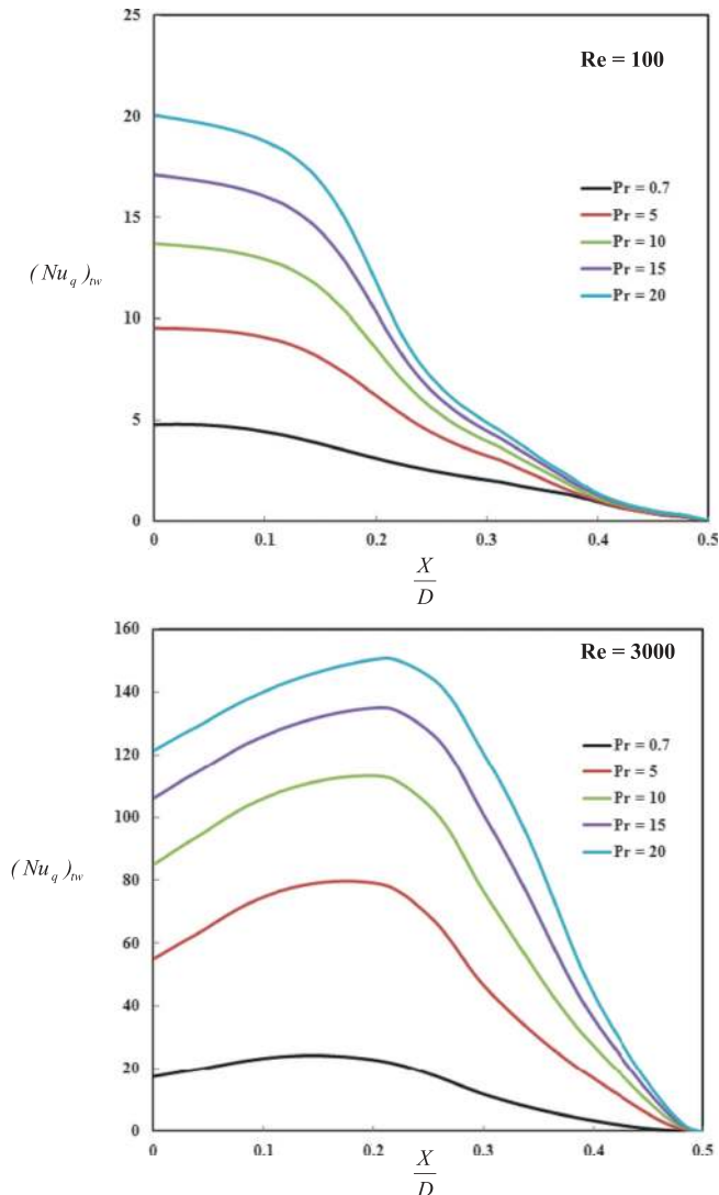
Figure 12. Local heat transfer solution at wall (cb) for H = 2.5 .
