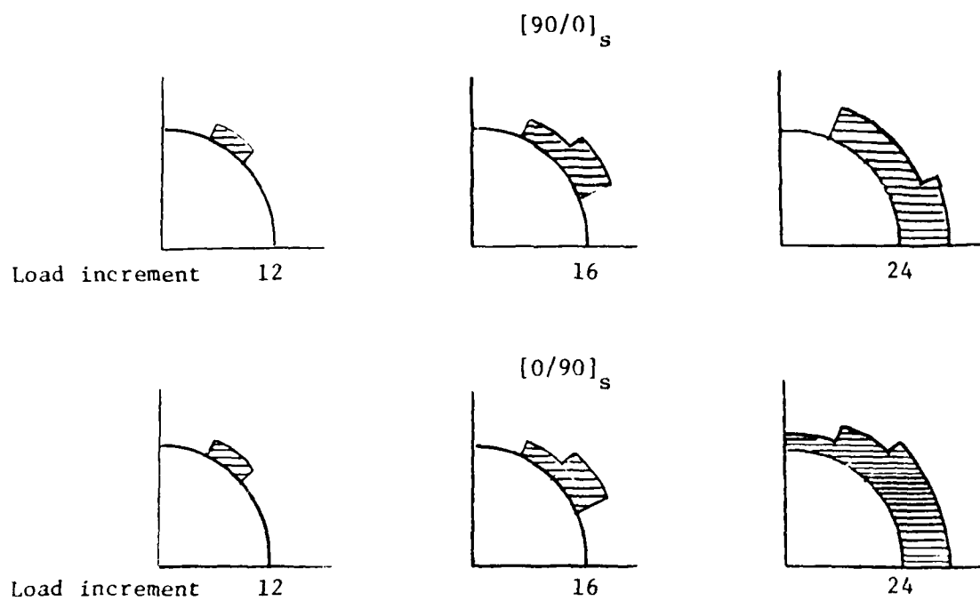
a) Propagation of yield zone in 0° ply
