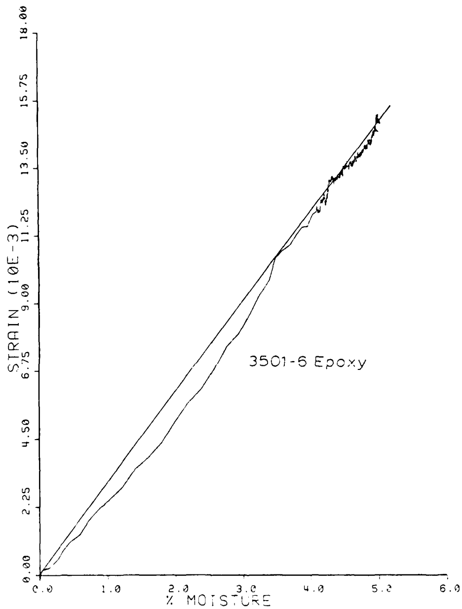
Figure 12. Results of Test 5, Station 2, 30 days @ 98% RH, 65.5°C (150°F).
