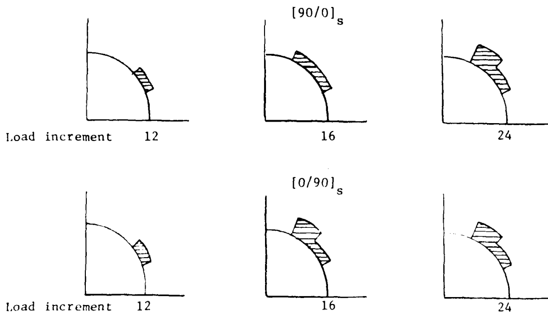
b) Propagation of yield zone in 90° ply
