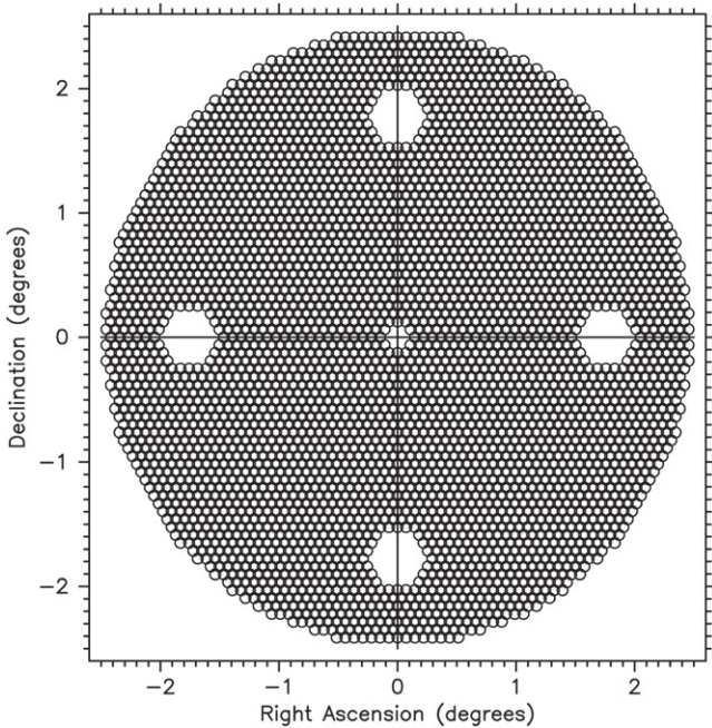
Figure 1. Configuration of the 4000 fiber positioning units covering the 5^\circ focal plane. The fibers are homogeneously distributed on the focal plane, except for the position of the active optics wave front sensor (central hole) and four Guiding CCD cameras (off-center holes).
