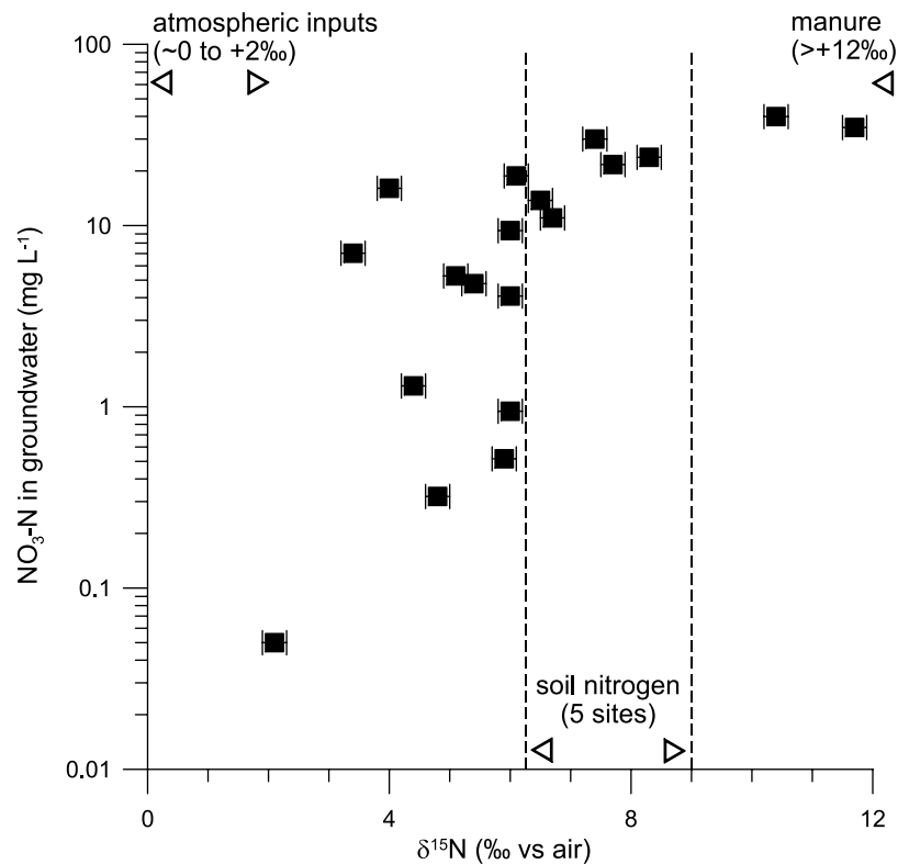
Figure 10. Isotopic values of nitrate in groundwater for a wide range of contents ( 0.05\text{--}40\text{ mg L}^{-1} , \text{NO}_3\text{-N} ). The local range in the mean \delta^{15}\text{N} values of five sampled soils (0–20 cm, 22 samples, total nitrogen) is also reported.
