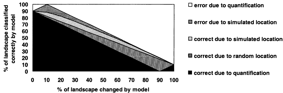
Fig. 4. Range for percent of landscape classified correctly by a model as a function of percent of landscape changed in a modeled scenario, where 10% of landscape is changed in reality.
