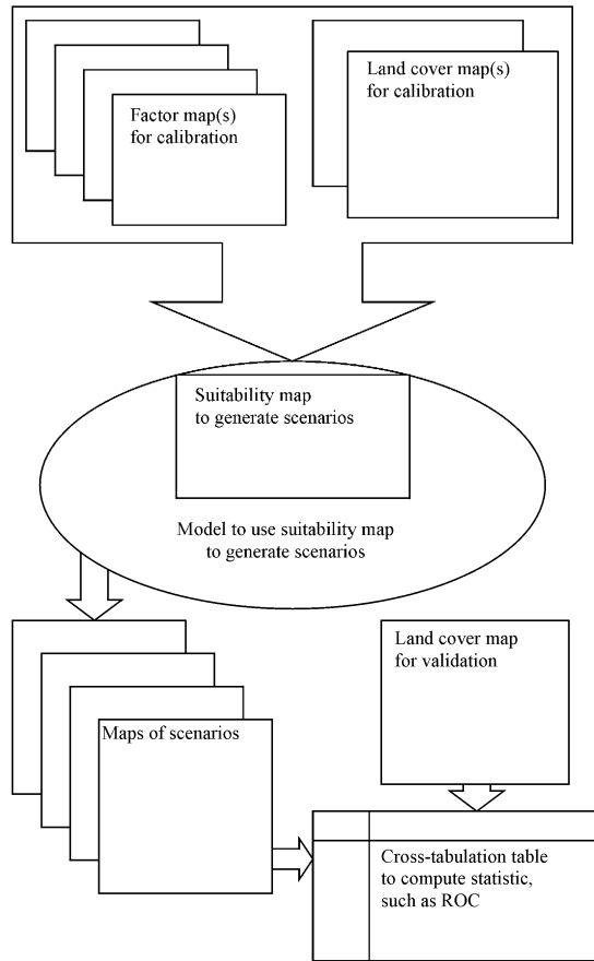
Fig. 1. Flow of logic among components necessary to validate a land-cover change model.
