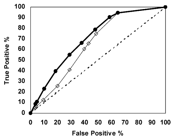
Fig. 5. ROC curves to validate models of deforestation in the Ipswich watershed between 1985 and 1991 using three suitability maps based on: random location (bottom ROC = 50%), logistic regression with protected areas (middle ROC = 65%), and MCE with a spatial filter and protected areas (upper ROC = 70%).
