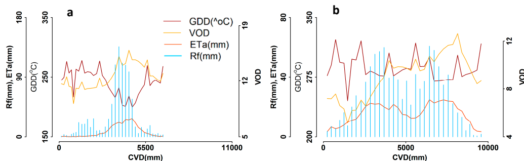
Figure 9. Time series of MODIS rainfall, SSEB ETa, and AMSR GDD and VOD for (a) #87 in Ethiopia and (b) #14 in Tanzania for 2003–2015.
