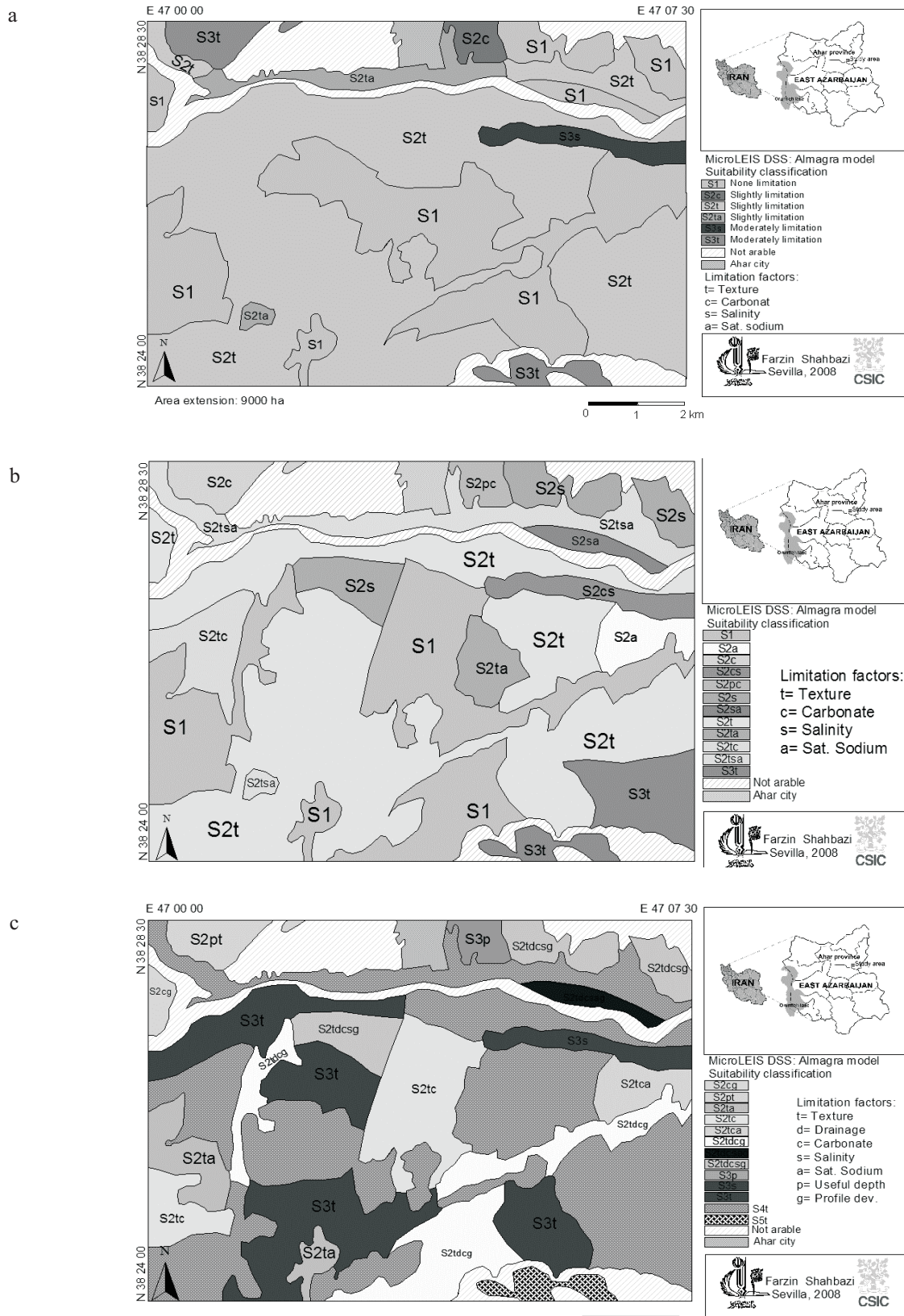
Fig. 5. Land suitability map of: a – wheat, b – alfalfa, and c – peach for Ahar province.
