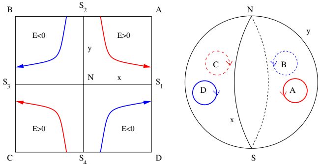
FIG. 2 (color online). Left: xy plane with the classical trajectories xy = E\ell^2 . Right: sphere that results from the identifications of the edges. Now the open trajectories become closed trajectories in one of four segments, enclosing one of the equatorial points A, B, C, D .
