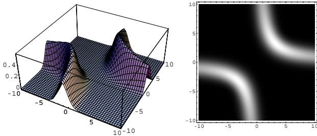
FIG. 1 (color online). Absolute value of the wave function \psi_E^+(x, y) for E = 10 in the interval -10 < x, y < 10 . The picture on the left gives a 3D representation while that on the right is a density plot.
