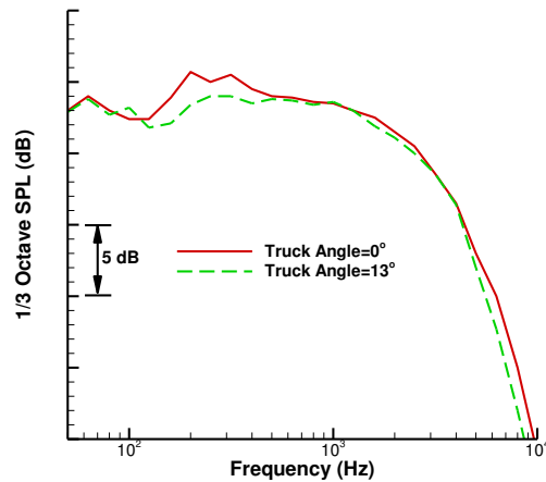
Figure 8 QTD2 test data showing the effects of landing gear truck angle.
