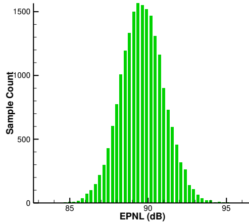
Figure 31. Sample count histogram of Monte Carlo simulation.
