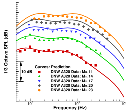
Figure 14. Validation by DNW Airbus 320 4-wheel full scale gear data.
